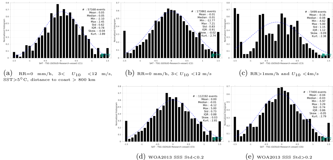
Figure 13: Normalized histogram of \Delta\text{SSS} (SMOS SSS L2 v700 (ESA) - TSG (GOSUD-Research-vessel)) for 5 different subdatasets corresponding to: RR=0 mm/h, 3 < U_{10} < 12 m/s, SST>5°C, distance to coast > 800 km (a), RR=0 mm/h, 3 < U_{10} < 12 m/s (b), RR>1mm/h and U_{10} < 4 m/s (c), WOA2013 SSS Std<0.2 (d), WOA2013 SSS Std>0.2 (e).
