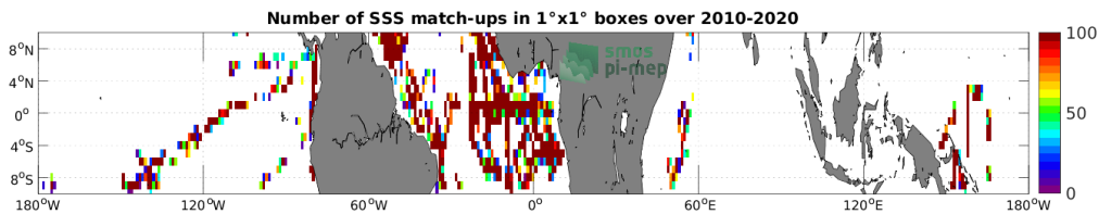
Figure 4: Number of SSS match-ups between TSG (GOSUD-Research-vessel) SSS and the SMOS SSS L2 v700 (ESA) SSS product for the Equatorial Ocean 10N-10S Pi-MEP region over 1^\circ \times 1^\circ boxes and for the full satellite product period.
