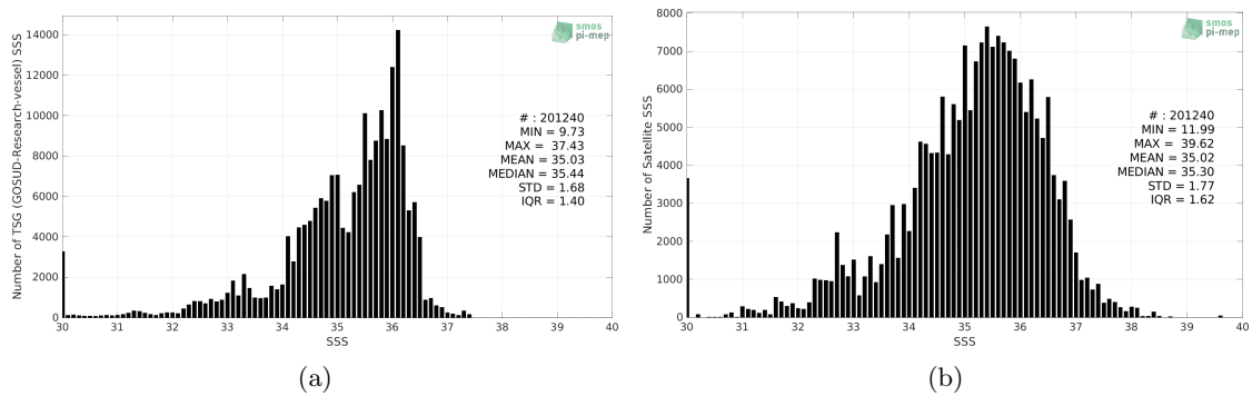
Figure 2: Histograms of SSS from TSG (GOSUD-Research-vessel) (a) and SMOS SSS L2 v700 (ESA) (b) considering all match-up pairs per bins of 0.1 over the Equatorial Ocean 10N-10S Pi-MEP region and for the full satellite product period.
