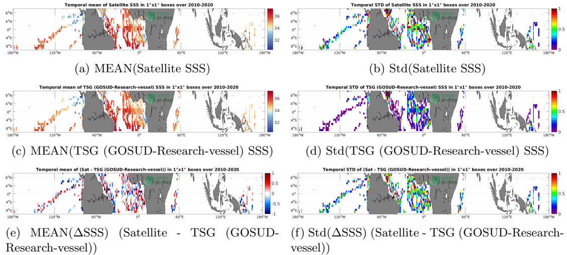
Figure 6: Temporal mean (left) and Std (right) of SSS from SMOS SSS L2 v700 (ESA) (top), TSG (GOSUD-Research-vessel) (middle), and of \Delta SSS (Satellite - TSG (GOSUD-Research-vessel)). Only match-up pairs are used to generate these maps.
