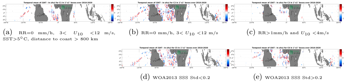
Figure 12: Temporal mean gridded over spatial boxes of size 1^\circ \times 1^\circ of \Delta SSS (SMOS SSS L2 v700 (ESA) - TSG (GOSUD-Research-vessel)) for 5 different subdatasets corresponding to: RR=0 mm/h, 3 < U_{10} < 12 m/s, SST>5°C, distance to coast > 800 km (a), RR=0 mm/h, 3 < U_{10} < 12 m/s (b), RR>1mm/h and U_{10} < 4 m/s (c), WOA2013 SSS Std<0.2 (d), WOA2013 SSS Std>0.2 (e).
