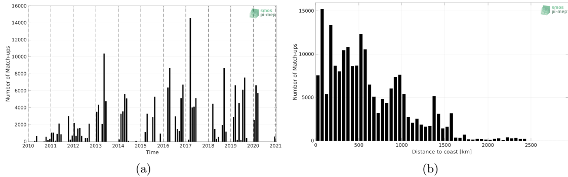
Figure 1: Number of match-ups between TSG (GOSUD-Research-vessel) and SMOS SSS L2 v700 (ESA) SSS as a function of time (a) and as function of the distance to coast (b) over the Equatorial Ocean 10N-10S Pi-MEP region and for the full satellite product period.
