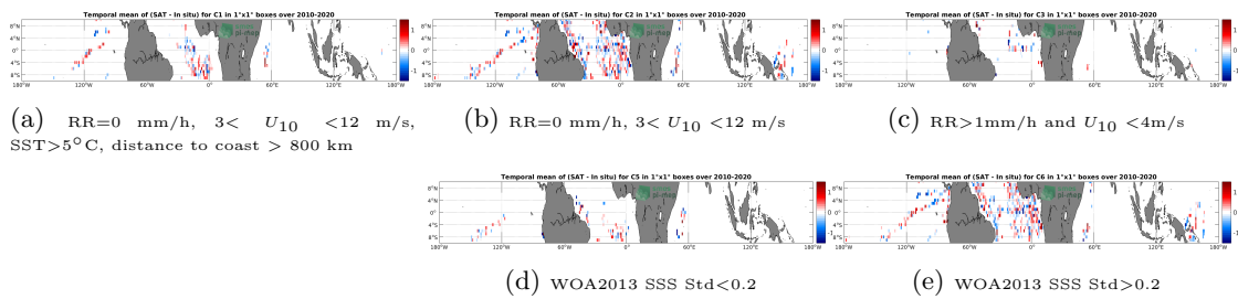
Figure 12: Temporal mean gridded over spatial boxes of size 1^\circ \times 1^\circ of \Delta SSS (SMOS SSS L2 v700 (ESA) - TSG (GOSUD-Research-vessel)) for 5 different subdatasets corresponding to: RR=0 mm/h, 3 < U_{10} < 12 m/s, SST>5°C, distance to coast > 800 km (a), RR=0 mm/h, 3 < U_{10} < 12 m/s (b), RR>1mm/h and U_{10} < 4 m/s (c), WOA2013 SSS Std<0.2 (d), WOA2013 SSS Std>0.2 (e).
