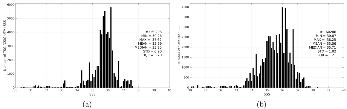
Figure 3: Histograms of SSS from TSG (CSIC-UTM) (a) and SMOS SSS L2 v700 (ESA) (b) considering all match-up pairs per bins of 0.1 over the Equatorial Ocean 10N-10S Pi-MEP region and for the full satellite product period.
