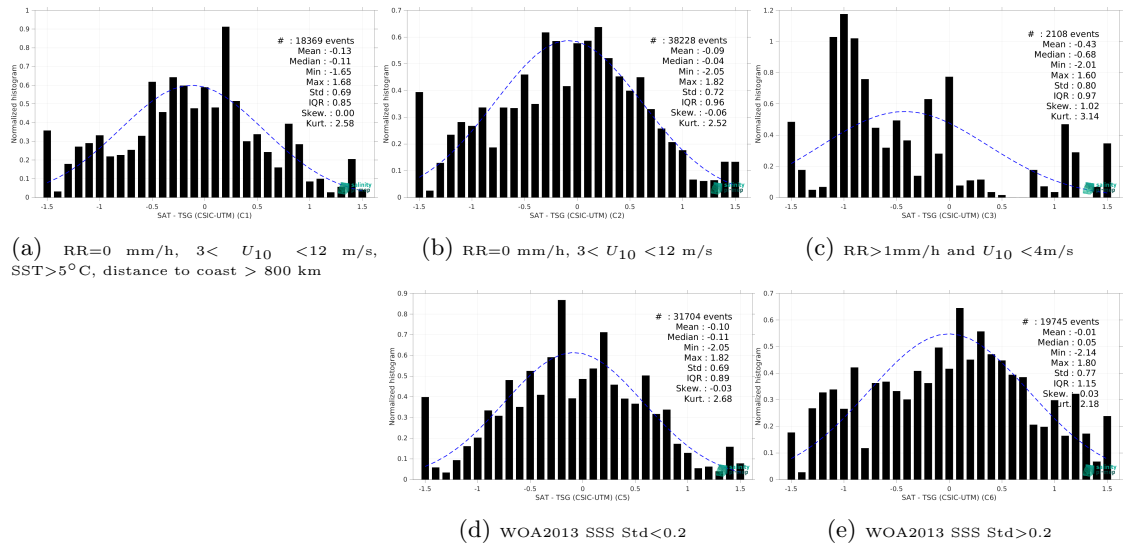
Figure 15: Normalized histogram of \Delta SSS (SMOS SSS L2 v700 (ESA) - TSG (CSIC-UTM)) for 5 different subdatasets corresponding to: RR=0 mm/h, 3 < U_{10} < 12 m/s, SST>5°C, distance to coast > 800 km (a), RR=0 mm/h, 3 < U_{10} < 12 m/s (b), RR>1mm/h and U_{10} < 4 m/s (c), WOA2013 SSS Std<0.2 (d), WOA2013 SSS Std>0.2 (e).
