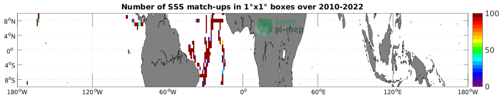
Figure 4: Number of SSS match-ups between TSG (CSIC-UTM) SSS and the SMOS SSS L2 v700 (ESA) SSS product for the Equatorial Ocean 10N-10S Pi-MEP region over 1^\circ \times 1^\circ boxes and for the full satellite product period.
