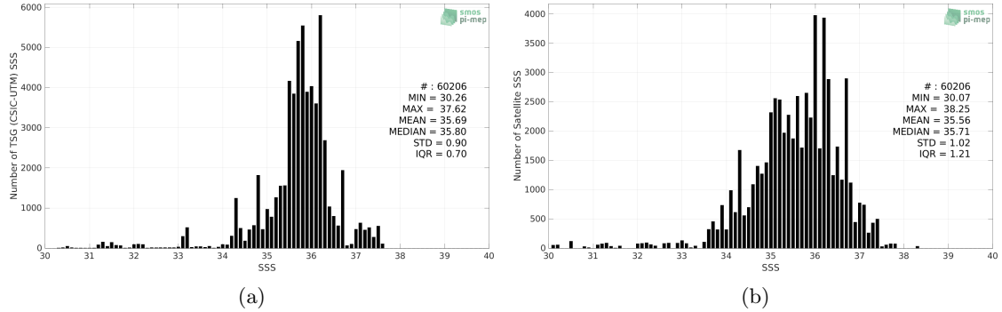
Figure 2: Histograms of SSS from TSG (CSIC-UTM) (a) and SMOS SSS L2 v700 (ESA) (b) considering all match-up pairs per bins of 0.1 over the Equatorial Ocean 10N-10S Pi-MEP region and for the full satellite product period.
