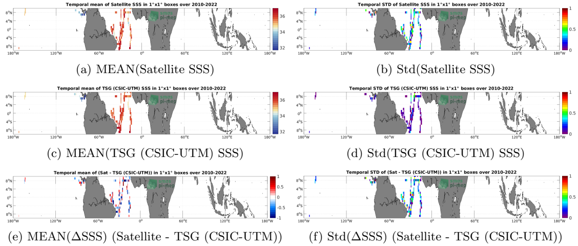
Figure 6: Temporal mean (left) and Std (right) of SSS from SMOS SSS L2 v700 (ESA) (top), TSG (CSIC-UTM) (middle), and of \Delta SSS (Satellite - TSG (CSIC-UTM)). Only match-up pairs are used to generate these maps.
