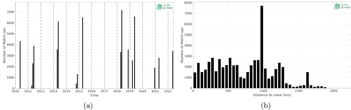
Figure 1: Number of match-ups between TSG (CSIC-UTM) and SMOS SSS L2 v700 (ESA) SSS as a function of time (a) and as function of the distance to coast (b) over the Equatorial Ocean 10N-10S Pi-MEP region and for the full satellite product period.
