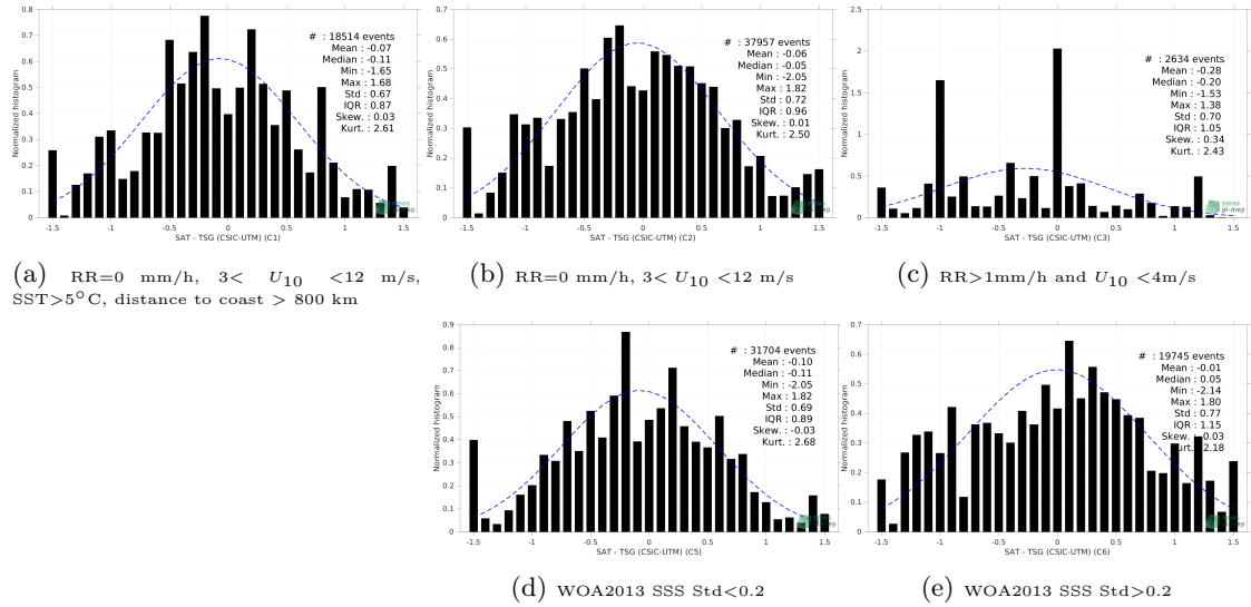
Figure 13: Normalized histogram of \Delta SSS (SMOS SSS L2 v700 (ESA) - TSG (CSIC-UTM)) for 5 different subdatasets corresponding to: RR=0 mm/h, 3 < U_{10} < 12 m/s, SST > 5^\circ C , distance to coast > 800 km (a), RR=0 mm/h, 3 < U_{10} < 12 m/s (b), RR>1mm/h and U_{10} < 4 m/s (c), WOA2013 SSS Std<0.2 (d), WOA2013 SSS Std>0.2 (e).
