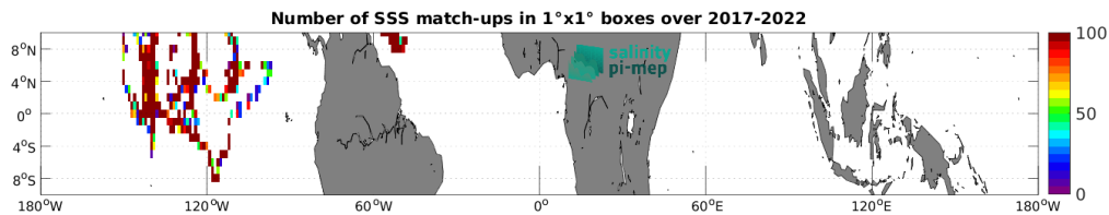
Figure 5: Number of SSS match-ups between Saildrone SSS and the SMOS SSS L2 v700 (ESA) SSS product for the Equatorial Ocean 10N-10S Pi-MEP region over 1^\circ \times 1^\circ boxes and for the full satellite product period.
