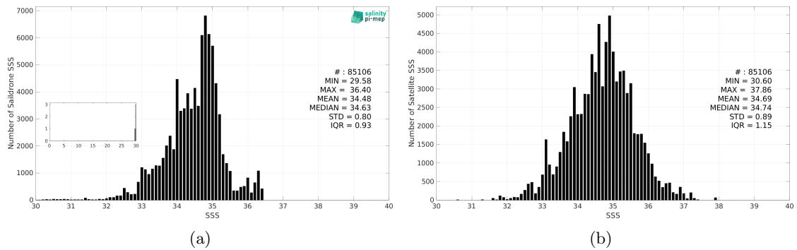
Figure 3: Histograms of SSS from Saildrone (a) and SMOS SSS L2 v700 (ESA) (b) considering all match-up pairs per bins of 0.1 over the Equatorial Ocean 10N-10S Pi-MEP region and for the full satellite product period.
