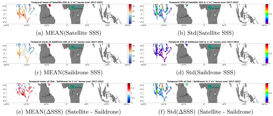
Figure 7: Temporal mean (left) and Std (right) of SSS from SMOS SSS L2 v700 (ESA) (top), Saildrone (middle), and of \Delta SSS (Satellite - Saildrone). Only match-up pairs are used to generate these maps.
