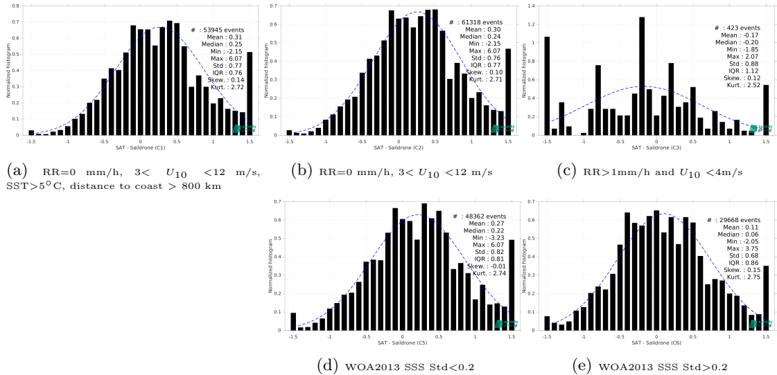
Figure 15: Normalized histogram of \Delta SSS (SMOS SSS L2 v700 (ESA) - Saildrone) for 5 different subdatasets corresponding to: RR=0 mm/h, 3 < U_{10} < 12 m/s, SST>5°C, distance to coast > 800 km (a), RR=0 mm/h, 3 < U_{10} < 12 m/s (b), RR>1mm/h and U_{10} < 4 m/s (c), WOA2013 SSS Std<0.2 (d), WOA2013 SSS Std>0.2 (e).
