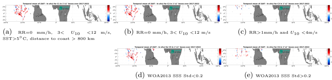
Figure 14: Temporal mean gridded over spatial boxes of size 1^\circ \times 1^\circ of \Delta SSS (SMOS SSS L2 v700 (ESA) - Saildrone) for 5 different subdatasets corresponding to:RR=0 mm/h, 3 < U_{10} < 12 m/s, SST>5°C, distance to coast > 800 km (a), RR=0 mm/h, 3 < U_{10} < 12 m/s (b), RR>1mm/h and U_{10} < 4 m/s (c), WOA2013 SSS Std<0.2 (d), WOA2013 SSS Std>0.2 (e).
