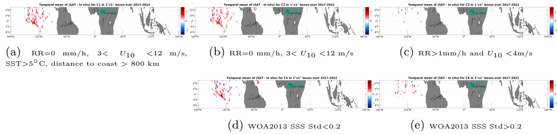
Figure 12: Temporal mean gridded over spatial boxes of size 1^\circ \times 1^\circ of \Delta SSS (SMOS SSS L2 v700 (ESA) - Sailldrone) for 5 different subdatasets corresponding to:RR=0 mm/h, 3 < U_{10} < 12 m/s, SST>5°C, distance to coast > 800 km (a), RR=0 mm/h, 3 < U_{10} < 12 m/s (b), RR>1mm/h and U_{10} < 4 m/s (c), WOA2013 SSS Std<0.2 (d), WOA2013 SSS Std>0.2 (e).
