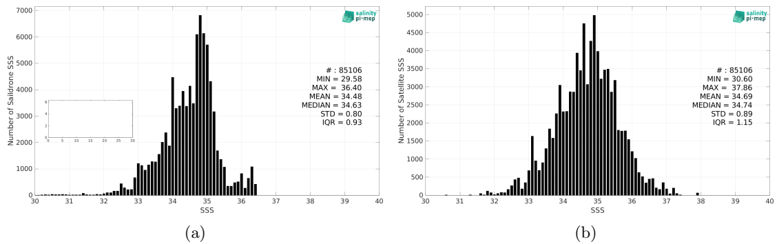
Figure 2: Histograms of SSS from Saildrone (a) and SMOS SSS L2 v700 (ESA) (b) considering all match-up pairs per bins of 0.1 over the Equatorial Ocean 10N-10S Pi-MEP region and for the full satellite product period.
