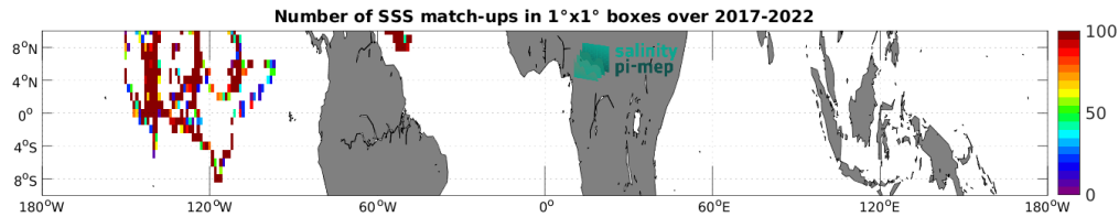
Figure 4: Number of SSS match-ups between Saildrone SSS and the SMOS SSS L2 v700 (ESA) SSS product for the Equatorial Ocean 10N-10S Pi-MEP region over 1^\circ \times 1^\circ boxes and for the full satellite product period.
