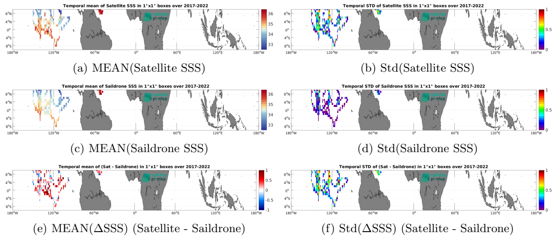
Figure 6: Temporal mean (left) and Std (right) of SSS from SMOS SSS L2 v700 (ESA) (top), Saildrone (middle), and of \Delta SSS (Satellite - Saildrone). Only match-up pairs are used to generate these maps.
