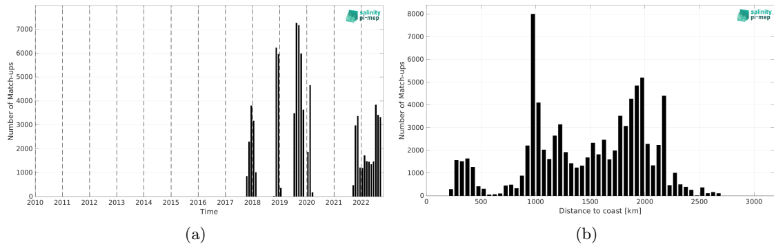
Figure 1: Number of match-ups between Saildrone and SMOS SSS L2 v700 (ESA) SSS as a function of time (a) and as function of the distance to coast (b) over the Equatorial Ocean 10N-10S Pi-MEP region and for the full satellite product period.
