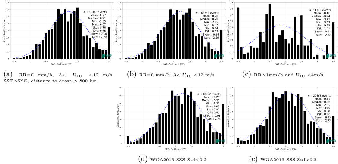
Figure 13: Normalized histogram of \Delta SSS (SMOS SSS L2 v700 (ESA) - Sailldrone) for 5 different subdatasets corresponding to: RR=0 mm/h, 3 < U_{10} < 12 m/s, SST>5°C, distance to coast > 800 km (a), RR=0 mm/h, 3 < U_{10} < 12 m/s (b), RR>1mm/h and U_{10} < 4 m/s (c), WOA2013 SSS Std<0.2 (d), WOA2013 SSS Std>0.2 (e).
