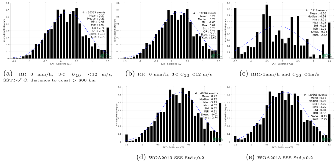
Figure 13: Normalized histogram of \Delta SSS (SMOS SSS L2 v700 (ESA) - Saiddrone) for 5 different subdatasets corresponding to: RR=0 mm/h, 3 < U_{10} < 12 m/s, SST >5^\circ\text{C} , distance to coast > 800 km (a), RR=0 mm/h, 3 < U_{10} < 12 m/s (b), RR >1 mm/h and U_{10} < 4 m/s (c), WOA2013 SSS Std <0.2 (d), WOA2013 SSS Std >0.2 (e).
