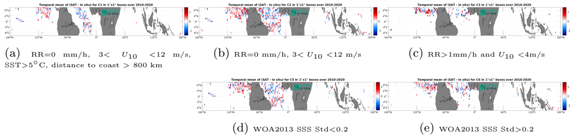
Figure 11: Temporal mean gridded over spatial boxes of size 1^\circ \times 1^\circ of \Delta SSS (SMOS SSS L2 v700 (ESA) - Surface drifters) for 5 different subdatasets corresponding to:RR=0 mm/h, 3 < U_{10} < 12 m/s, SST >5^\circ\text{C} , distance to coast > 800 km (a), RR=0 mm/h, 3 < U_{10} < 12 m/s (b), RR >1 mm/h and U_{10} < 4 m/s (c), WOA2013 SSS Std <0.2 (d), WOA2013 SSS Std >0.2 (e).
