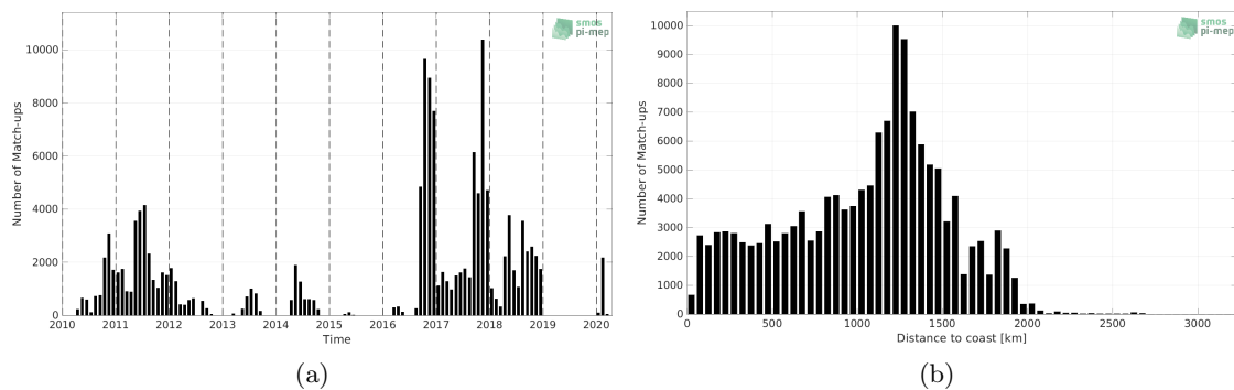
Figure 1: Number of match-ups between Surface drifters and SMOS SSS L2 v700 (ESA) SSS as a function of time (a) and as function of the distance to coast (b) over the Equatorial Ocean 10N-10S Pi-MEP region and for the full satellite product period.
