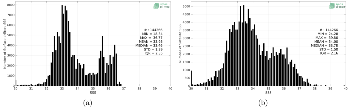
Figure 2: Histograms of SSS from Surface drifters (a) and SMOS SSS L2 v700 (ESA) (b) considering all match-up pairs per bins of 0.1 over the Equatorial Ocean 10N-10S Pi-MEP region and for the full satellite product period.
