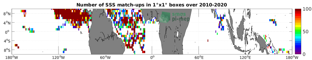
Figure 3: Number of SSS match-ups between Surface drifters SSS and the SMOS SSS L2 v700 (ESA) SSS product for the Equatorial Ocean 10N-10S Pi-MEP region over 1^\circ \times 1^\circ boxes and for the full satellite product period.
