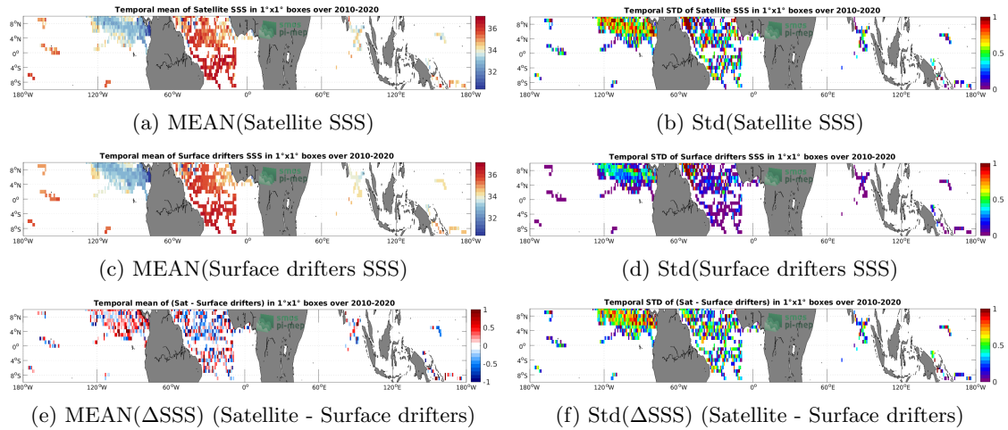
Figure 5: Temporal mean (left) and Std (right) of SSS from SMOS SSS L2 v700 (ESA) (top), Surface drifters (middle), and of \Delta SSS (Satellite - Surface drifters). Only match-up pairs are used to generate these maps.
