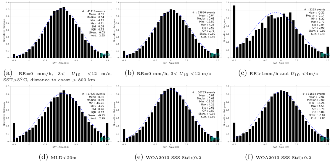
Figure 13: Normalized histogram of \Delta SSS (SMOS SSS L2 v700 (ESA) - Argo) for 6 different subdatasets corresponding to: RR=0 mm/h, 3 < U_{10} < 12 m/s, SST >5^\circ C, distance to coast > 800 km (a), RR=0 mm/h, 3 < U_{10} < 12 m/s (b), RR >1 mm/h and U_{10} < 4 m/s (c), MLD <20 m (d), WOA2013 SSS Std <0.2 (e), WOA2013 SSS Std >0.2 (f).
