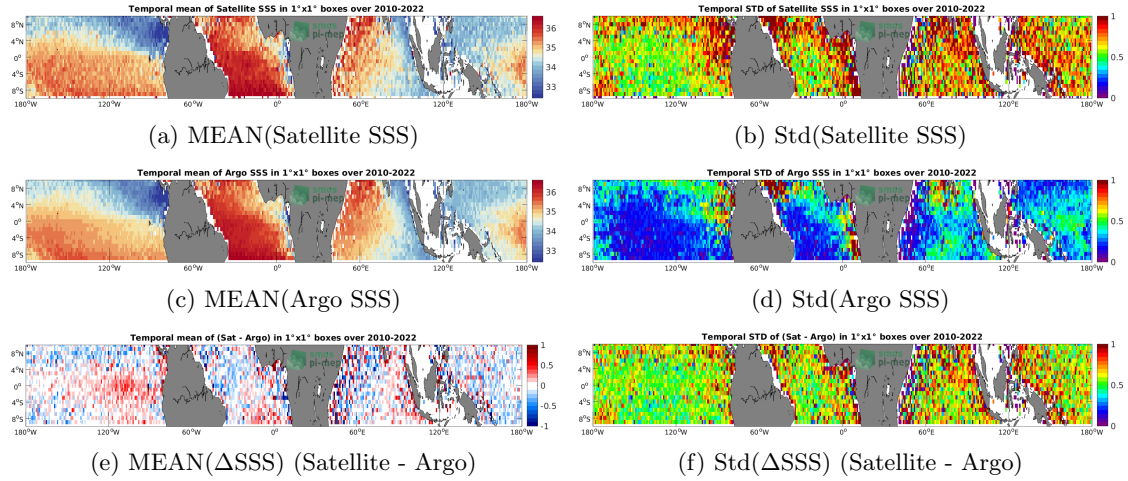
Figure 6: Temporal mean (left) and Std (right) of SSS from SMOS SSS L2 v700 (ESA) (top), Argo (middle), and of \Delta SSS (Satellite - Argo). Only match-up pairs are used to generate these maps.
