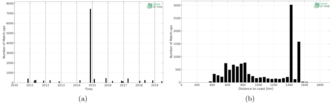
Figure 1: Number of match-ups between TSG (Polarstern) and SMOS SSS L2 v662 (ESA) SSS as a function of time (a) and as function of the distance to coast (b) over the Equatorial Ocean 10N-10S Pi-MEP region and for the full satellite product period.
