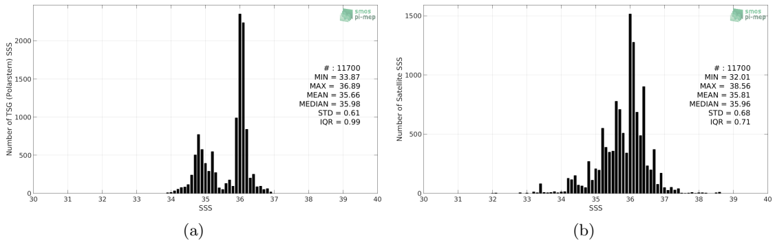
Figure 2: Histograms of SSS from TSG (Polarstern) (a) and SMOS SSS L2 v662 (ESA) (b) considering all match-up pairs per bins of 0.1 over the Equatorial Ocean 10N-10S Pi-MEP region and for the full satellite product period.
