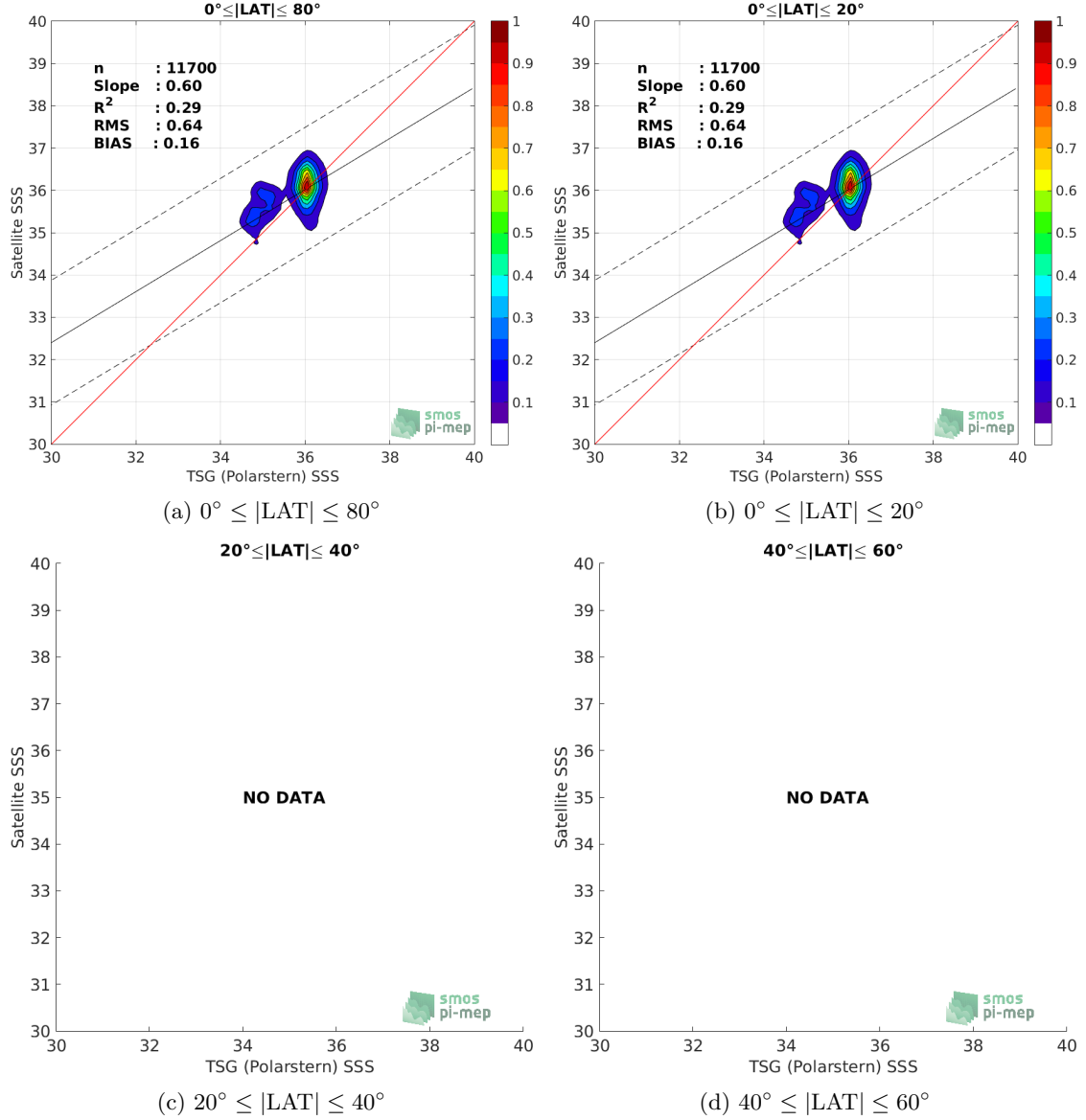
Figure 9: Contour maps of the concentration of SMOS SSS L2 v662 (ESA) SSS (y-axis) versus TSG (Polarstern) SSS (x-axis) at match-up pairs for different latitude bands. For each plot, the red line shows x=y . The black thin and dashed lines indicate a linear fit through the data cloud and the \pm 95\% confidence levels, respectively. The number match-up pairs n , the slope and R^2 coefficient of the linear fit, the root mean square (RMS) and the mean bias between satellite and in situ data are indicated for each latitude band in each plots.
