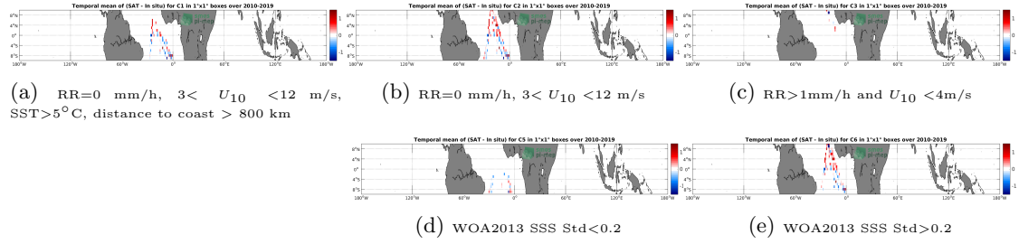
Figure 12: Temporal mean gridded over spatial boxes of size 1^\circ \times 1^\circ of \Delta SSS (SMOS SSS L2 v662 (ESA) - TSG (Polarstern)) for 5 different subdatasets corresponding to:RR=0 mm/h, 3 < U_{10} < 12 m/s, SST >5^\circ\text{C} , distance to coast > 800 km (a), RR=0 mm/h, 3 < U_{10} < 12 m/s (b), RR >1 mm/h and U_{10} < 4 m/s (c), WOA2013 SSS Std <0.2 (d), WOA2013 SSS Std >0.2 (e).
