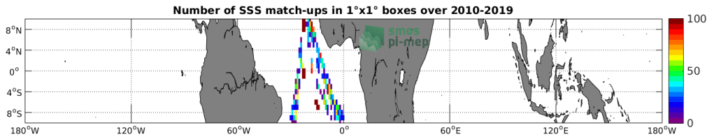
Figure 4: Number of SSS match-ups between TSG (Polarstern) SSS and the SMOS SSS L2 v662 (ESA) SSS product for the Equatorial Ocean 10N-10S Pi-MEP region over 1^\circ \times 1^\circ boxes and for the full satellite product period.
