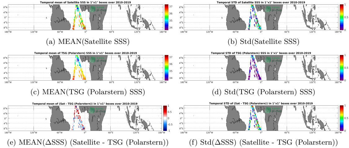
Figure 6: Temporal mean (left) and Std (right) of SSS from SMOS SSS L2 v662 (ESA) (top), TSG (Polarstern) (middle), and of \Delta SSS (Satellite - TSG (Polarstern)). Only match-up pairs are used to generate these maps.
