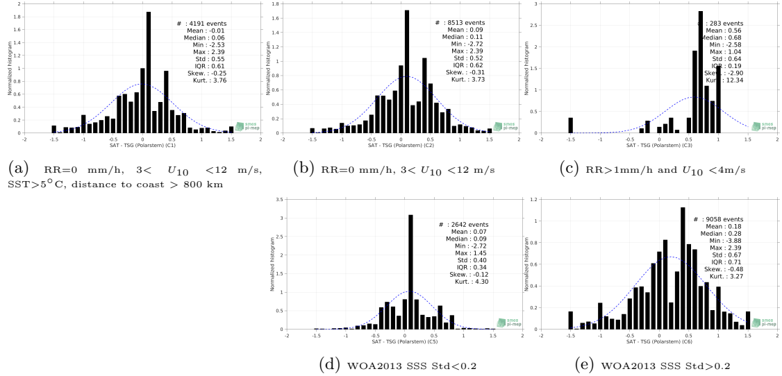
Figure 13: Normalized histogram of \Delta SSS (SMOS SSS L2 v662 (ESA) - TSG (Polarstern)) for 5 different subdatasets corresponding to: RR=0 mm/h, 3 < U_{10} < 12 m/s, SST >5^\circ\text{C} , distance to coast > 800 km (a), RR=0 mm/h, 3 < U_{10} < 12 m/s (b), RR >1 mm/h and U_{10} < 4 m/s (c), WOA2013 SSS Std <0.2 (d), WOA2013 SSS Std >0.2 (e).
