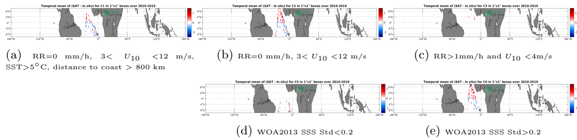
Figure 12: Temporal mean gridded over spatial boxes of size 1^\circ \times 1^\circ of \Delta SSS (SMOS SSS L2 v662 (ESA) - TSG (Polarstern)) for 5 different subdatasets corresponding to: RR=0 mm/h, 3 < U_{10} < 12 m/s, SST > 5^\circ C , distance to coast > 800 km (a), RR=0 mm/h, 3 < U_{10} < 12 m/s (b), RR > 1 mm/h and U_{10} < 4 m/s (c), WOA2013 SSS Std < 0.2 (d), WOA2013 SSS Std > 0.2 (e).
