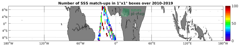
Figure 4: Number of SSS match-ups between TSG (Polarstern) SSS and the SMOS SSS L2 v662 (ESA) SSS product for the Equatorial Ocean 10N-10S Pi-MEP region over 1°x1° boxes and for the full satellite product period.
