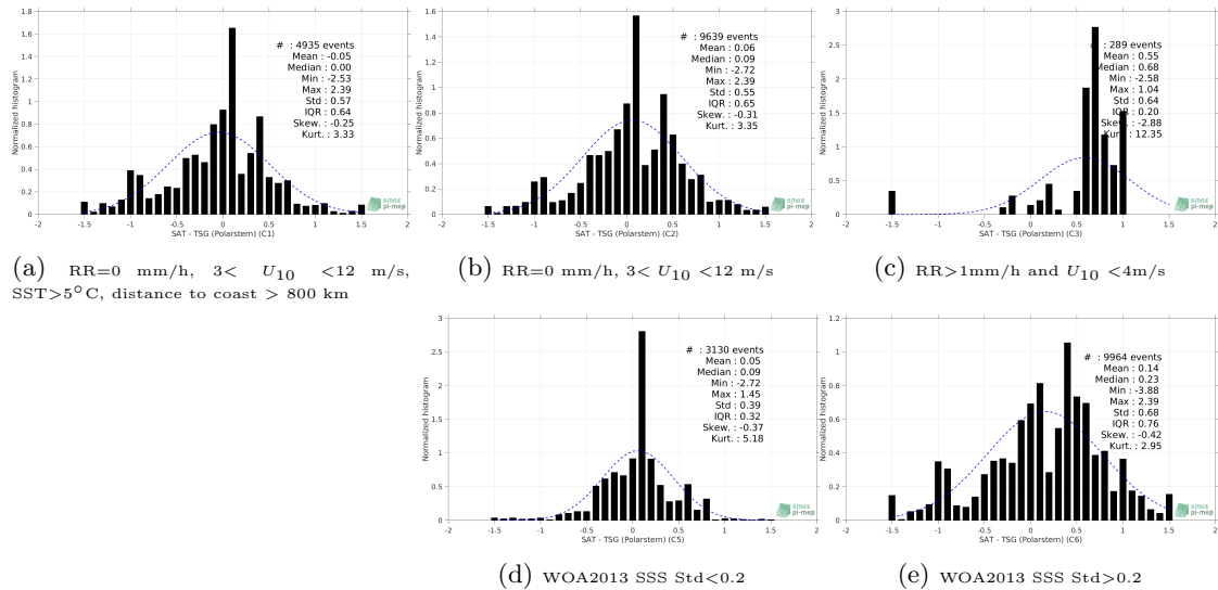
Figure 13: Normalized histogram of \Delta SSS (SMOS SSS L2 v662 (ESA) - TSG (Polarstern)) for 5 different subdatasets corresponding to: RR=0 mm/h, 3 < U_{10} < 12 m/s, SST > 5^\circ C , distance to coast > 800 km (a), RR=0 mm/h, 3 < U_{10} < 12 m/s (b), RR > 1 mm/h and U_{10} < 4 m/s (c), WOA2013 SSS Std < 0.2 (d), WOA2013 SSS Std > 0.2 (e).
