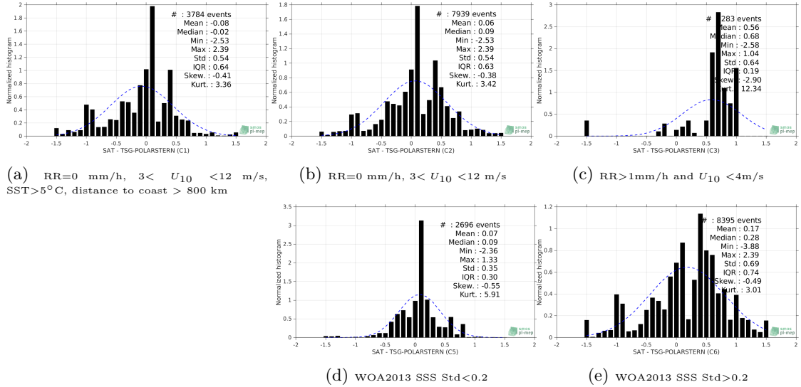
Figure 13: Normalized histogram of \Delta SSS (SMOS-L2-DPGS-v662 - TSG-POLARSTERN) for 5 different subdatasets corresponding to: RR=0 mm/h, 3 < U_{10} < 12 m/s, SST > 5^\circ C , distance to coast > 800 km (a), RR=0 mm/h, 3 < U_{10} < 12 m/s (b), RR > 1 mm/h and U_{10} < 4 m/s (c), WOA2013 SSS Std < 0.2 (d), WOA2013 SSS Std > 0.2 (e).
