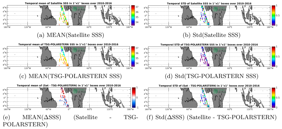
Figure 6: Temporal mean (left) and Std (right) of SSS from SMOS-L2-DPGS-v662 (top), TSG-POLARSTERN (middle), and of \Delta SSS (Satellite - TSG-POLARSTERN). Only match-up pairs are used to generate these maps.
