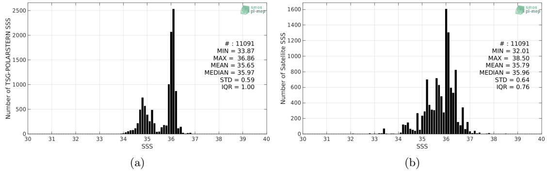
Figure 2: Histograms of SSS from TSG-POLARSTERN (a) and SMOS-L2-DPGS-v662 (b) considering all match-up pairs per bins of 0.1 over the Equatorial Ocean 10N-10S Pi-MEP region and for the full satellite product period.
