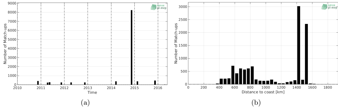
Figure 1: Number of match-ups between TSG-POLARSTERN and SMOS-L2-DPGS-v662 SSS as a function of time (a) and as function of the distance to coast (b) over the Equatorial Ocean 10N-10S Pi-MEP region and for the full satellite product period.
