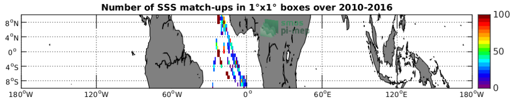
Figure 4: Number of SSS match-ups between TSG-POLARSTERN SSS and the SMOS-L2-DPGS-v662 SSS product for the Equatorial Ocean 10N-10S Pi-MEP region over 1^\circ \times 1^\circ boxes and for the full satellite product period.
