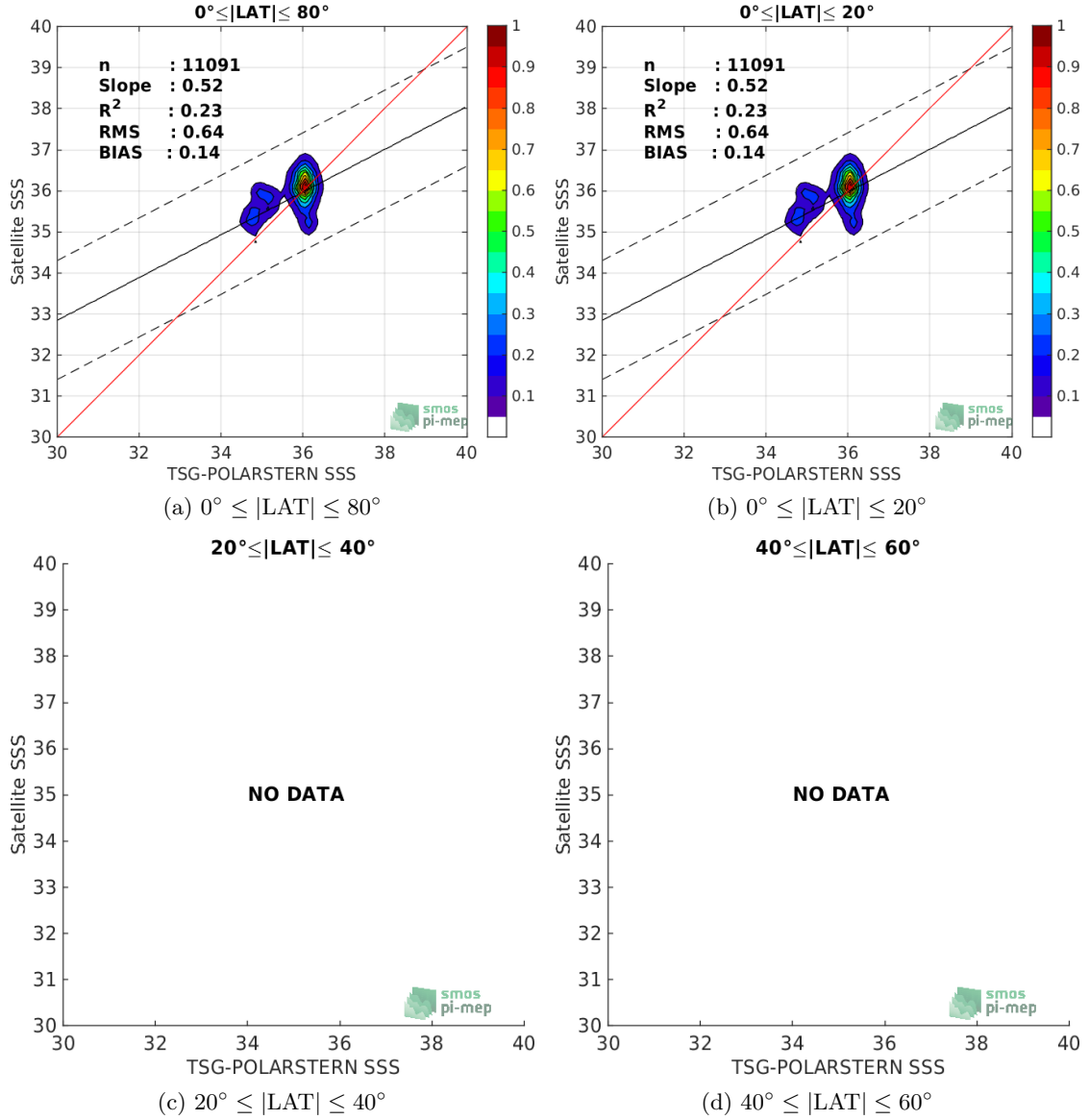
Figure 9: Contour maps of the concentration of SMOS-L2-DPGS-v662 SSS (y-axis) versus TSG-POLARSTERN SSS (x-axis) at match-up pairs for different latitude bands. For each plot, the red line shows x=y . The black thin and dashed lines indicate a linear fit through the data cloud and the \pm 95\% confidence levels, respectively. The number match-up pairs n , the slope and R^2 coefficient of the linear fit, the root mean square (RMS) and the mean bias between satellite and in situ data are indicated for each latitude band in each plots.
