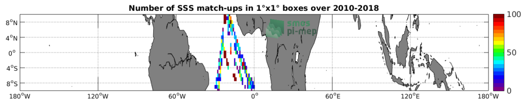
Figure 4: Number of SSS match-ups between TSG-POLARSTERN SSS and the SMOS-L2-DPGS-v662 SSS product for the Equatorial Ocean 10N-10S Pi-MEP region over 1^\circ \times 1^\circ boxes and for the full satellite product period.
