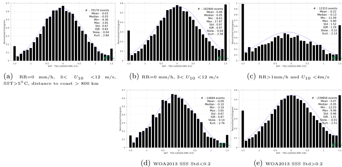
Figure 13: Normalized histogram of \Delta SSS (SMOS SSS L2 v662 (ESA) - TSG (LEGOS-DM)) for 5 different subdatasets corresponding to: RR=0 mm/h, 3 < U_{10} < 12 m/s, SST >5^\circ\text{C} , distance to coast > 800 km (a), RR=0 mm/h, 3 < U_{10} < 12 m/s (b), RR >1 mm/h and U_{10} < 4 m/s (c), WOA2013 SSS Std <0.2 (d), WOA2013 SSS Std >0.2 (e).
