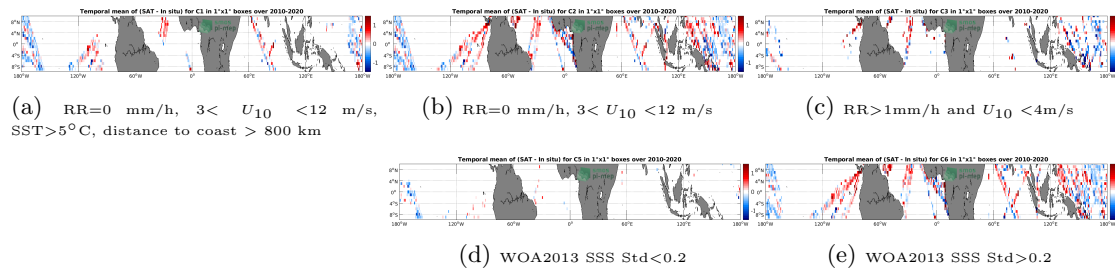
Figure 12: Temporal mean gridded over spatial boxes of size 1^\circ \times 1^\circ of \Delta SSS (SMOS SSS L2 v662 (ESA) - TSG (LEGOS-DM)) for 5 different subdatasets corresponding to:RR=0 mm/h, 3 < U_{10} < 12 m/s, SST >5^\circ\text{C} , distance to coast > 800 km (a), RR=0 mm/h, 3 < U_{10} < 12 m/s (b), RR >1 mm/h and U_{10} < 4 m/s (c), WOA2013 SSS Std <0.2 (d), WOA2013 SSS Std >0.2 (e).
