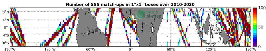
Figure 4: Number of SSS match-ups between TSG (LEGOS-DM) SSS and the SMOS SSS L2 v662 (ESA) SSS product for the Equatorial Ocean 10N-10S Pi-MEP region over 1^\circ \times 1^\circ boxes and for the full satellite product period.
