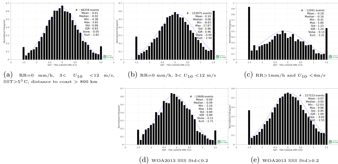
Figure 13: Normalized histogram of ΔSSS (SMOS SSS L2 v662 (ESA) - TSG (LEGOS-DM)) for 5 different subdatasets corresponding to: RR=0 mm/h, 3 < U_{10} < 12 m/s, SST>5°C, distance to coast > 800 km (a), RR=0 mm/h, 3 < U_{10} < 12 m/s (b), RR>1mm/h and U_{10} < 4m/s (c), WOA2013 SSS Std<0.2 (d), WOA2013 SSS Std>0.2 (e).
