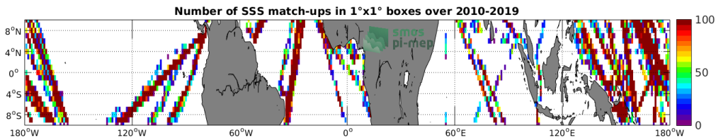
Figure 4: Number of SSS match-ups between TSG (LEGOS-DM) SSS and the SMOS SSS L2 v662 (ESA) SSS product for the Equatorial Ocean 10N-10S Pi-MEP region over 1°x1° boxes and for the full satellite product period.
