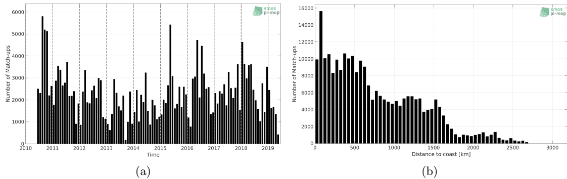
Figure 1: Number of match-ups between TSG (LEGOS-DM) and SMOS SSS L2 v662 (ESA) SSS as a function of time (a) and as function of the distance to coast (b) over the Equatorial Ocean 10N-10S Pi-MEP region and for the full satellite product period.
