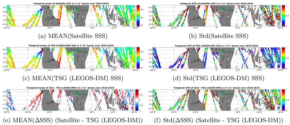
Figure 6: Temporal mean (left) and Std (right) of SSS from SMOS SSS L2 v662 (ESA) (top), TSG (LEGOS-DM) (middle), and of \Delta SSS (Satellite - TSG (LEGOS-DM)). Only match-up pairs are used to generate these maps.
