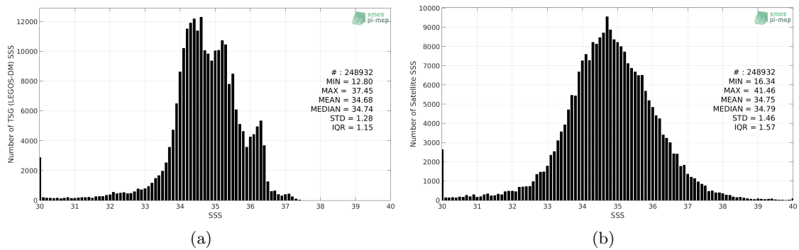
Figure 2: Histograms of SSS from TSG (LEGOS-DM) (a) and SMOS SSS L2 v662 (ESA) (b) considering all match-up pairs per bins of 0.1 over the Equatorial Ocean 10N-10S Pi-MEP region and for the full satellite product period.
