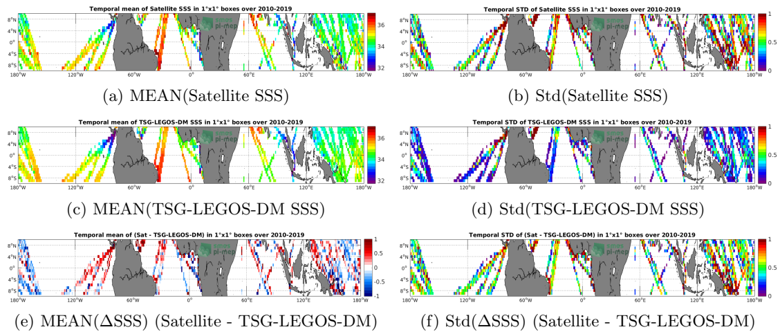
Figure 6: Temporal mean (left) and Std (right) of SSS from SMOS L2 v662 (ESA) (top), TSG-LEGOS-DM (middle), and of \Delta SSS (Satellite - TSG-LEGOS-DM). Only match-up pairs are used to generate these maps.
