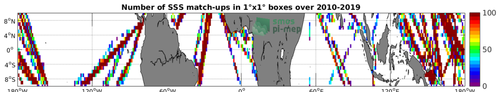
Figure 4: Number of SSS match-ups between TSG-LEGOS-DM SSS and the SMOS L2 v662 (ESA) SSS product for the Equatorial Ocean 10N-10S Pi-MEP region over 1^\circ \times 1^\circ boxes and for the full satellite product period.
