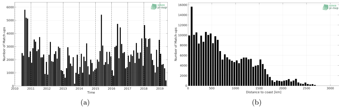
Figure 1: Number of match-ups between TSG-LEGOS-DM and SMOS L2 v662 (ESA) SSS as a function of time (a) and as function of the distance to coast (b) over the Equatorial Ocean 10N-10S Pi-MEP region and for the full satellite product period.
