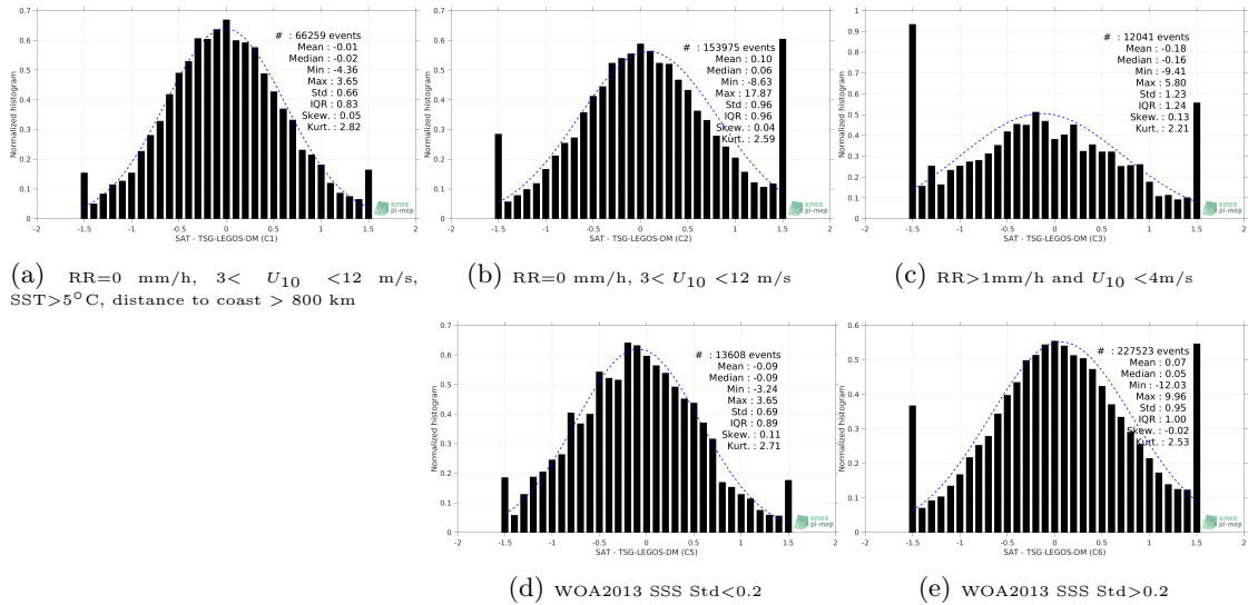
Figure 13: Normalized histogram of \Delta SSS (SMOS L2 v662 (ESA) - TSG-LEGOS-DM) for 5 different subdatasets corresponding to: RR=0 mm/h, 3 < U_{10} < 12 m/s, SST > 5^\circ C , distance to coast > 800 km (a), RR=0 mm/h, 3 < U_{10} < 12 m/s (b), RR > 1 mm/h and U_{10} < 4 m/s (c), WOA2013 SSS Std < 0.2 (d), WOA2013 SSS Std > 0.2 (e).
