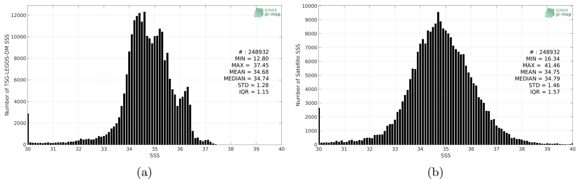
Figure 2: Histograms of SSS from TSG-LEGOS-DM (a) and SMOS L2 v662 (ESA) (b) considering all match-up pairs per bins of 0.1 over the Equatorial Ocean 10N-10S Pi-MEP region and for the full satellite product period.
