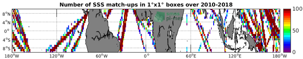
Figure 4: Number of SSS match-ups between TSG-LEGOS-DM SSS and the SMOS-L2-DPGS-v662 SSS product for the Equatorial Ocean 10N-10S Pi-MEP region over 1°x1° boxes and for the full satellite product period.
