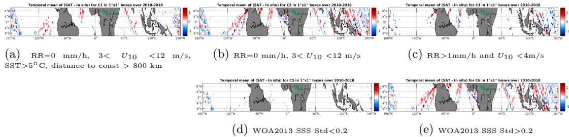
Figure 12: Temporal mean gridded over spatial boxes of size 1^\circ \times 1^\circ of \Delta SSS (SMOS-L2-DPGS-v662 - TSG-LEGOS-DM) for 5 different subdatasets corresponding to:RR=0 mm/h, 3 < U_{10} < 12 m/s, SST >5^\circ\text{C} , distance to coast > 800 km (a), RR=0 mm/h, 3 < U_{10} < 12 m/s (b), RR >1 mm/h and U_{10} < 4 m/s (c), WOA2013 SSS Std <0.2 (d), WOA2013 SSS Std >0.2 (e).
