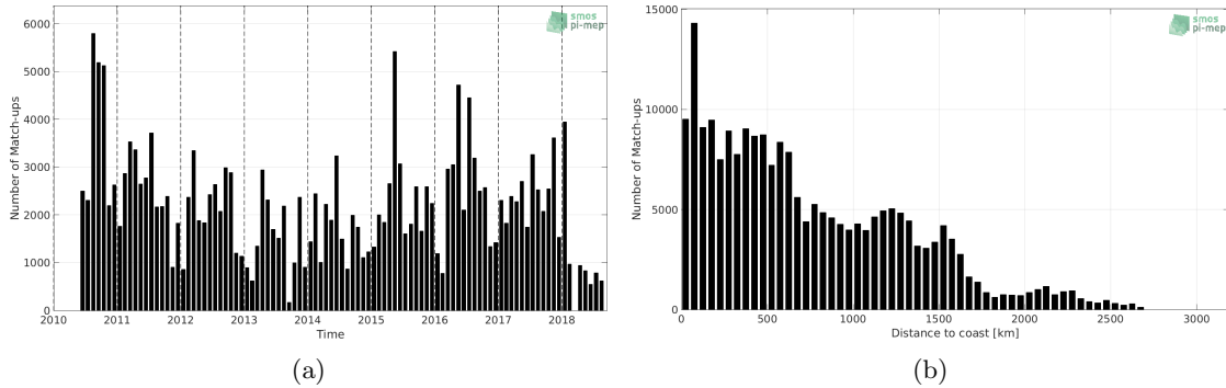
Figure 1: Number of match-ups between TSG-LEGOS-DM and SMOS-L2-DPGS-v662 SSS as a function of time (a) and as function of the distance to coast (b) over the Equatorial Ocean 10N-10S Pi-MEP region and for the full satellite product period.
