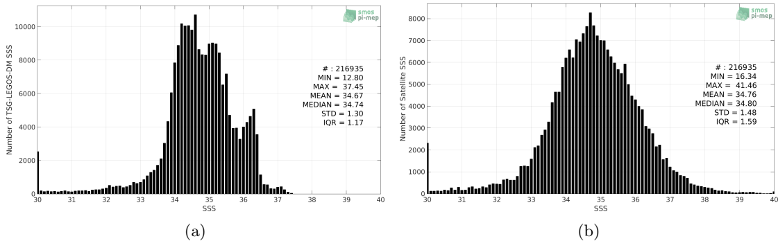
Figure 2: Histograms of SSS from TSG-LEGOS-DM (a) and SMOS-L2-DPGS-v662 (b) considering all match-up pairs per bins of 0.1 over the Equatorial Ocean 10N-10S Pi-MEP region and for the full satellite product period.
