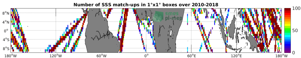
Figure 4: Number of SSS match-ups between TSG-LEGOS-DM SSS and the SMOS-L2-DPGS-v662 SSS product for the Equatorial Ocean 10N-10S Pi-MEP region over 1^\circ \times 1^\circ boxes and for the full satellite product period.
