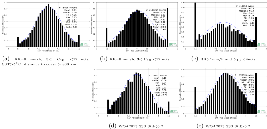
Figure 13: Normalized histogram of \Delta SSS (SMOS-L2-DPGS-v662 - TSG-LEGOS-DM) for 5 different subdatasets corresponding to: RR=0 mm/h, 3 < U_{10} < 12 m/s, SST >5^\circ\text{C} , distance to coast > 800 km (a), RR=0 mm/h, 3 < U_{10} < 12 m/s (b), RR >1 mm/h and U_{10} < 4 m/s (c), WOA2013 SSS Std <0.2 (d), WOA2013 SSS Std >0.2 (e).
