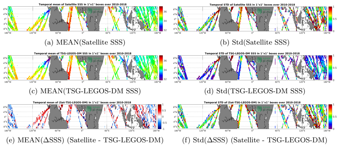
Figure 6: Temporal mean (left) and Std (right) of SSS from SMOS-L2-DPGS-v662 (top), TSG-LEGOS-DM (middle), and of \Delta SSS (Satellite - TSG-LEGOS-DM). Only match-up pairs are used to generate these maps.
