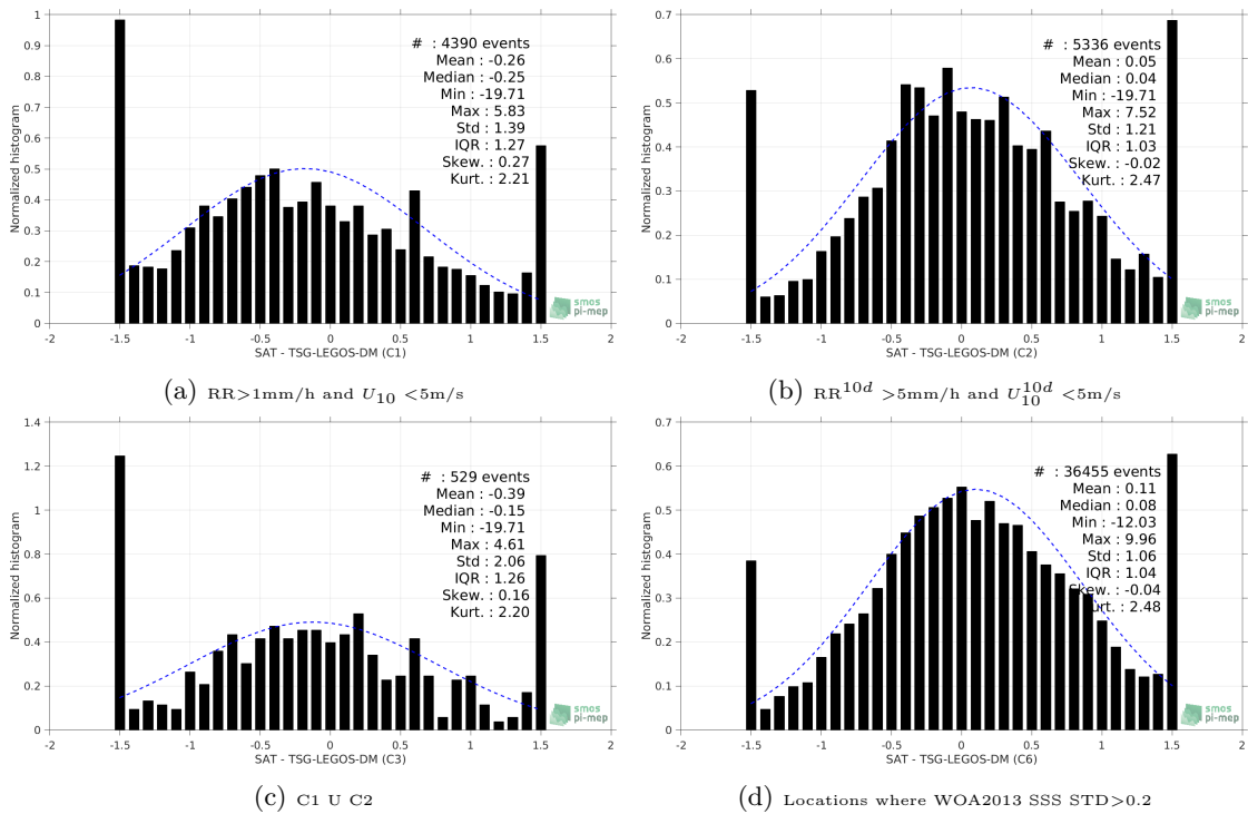
Figure 13: Normalized histogram of \Delta SSS (SMOS-L2-DPGS-v662 - TSG-LEGOS-DM) for 6 different subdatasets corresponding to: RR >1 mm/h and U_{10} < 5 m/s (a), RR ^{10d} > 5 mm/h and U_{10}^{10d} < 5 m/s (b), C1 U C2 (c), Locations where WOA2013 SSS STD >0.2 (d).
