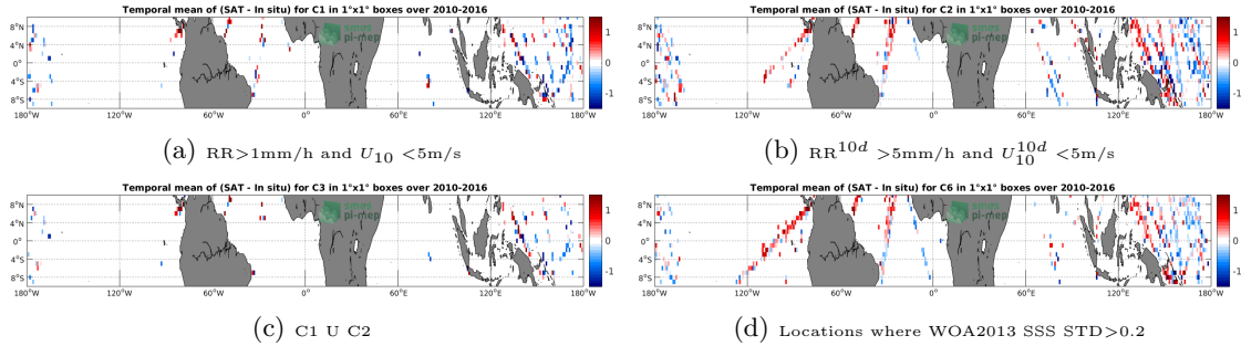
Figure 12: Temporal mean gridded over spatial boxes of size 1^\circ \times 1^\circ of \Delta SSS (SMOS-L2-DPGS-v662 - TSG-LEGOS-DM) for 4 different subdatasets corresponding to: RR >1 mm/h and U_{10} < 5 m/s (a), RR ^{10d} > 5 mm/h and U_{10}^{10d} < 5 m/s (b), C1 U C2 (c), Locations where WOA2013 SSS STD >0.2 (d).
