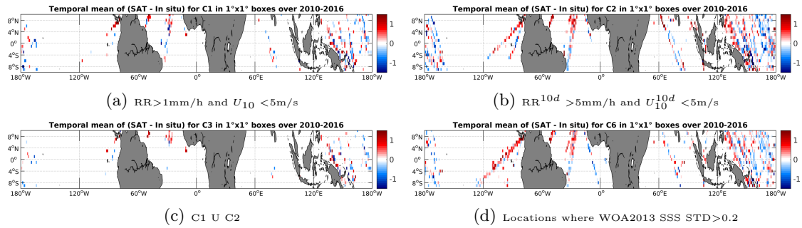
Figure 12: Temporal mean gridded over spatial boxes of size 1^\circ \times 1^\circ of \Delta SSS (SMOS-L2-DPGS-v662 - TSG-LEGOS-DM) for 4 different subdatasets corresponding to: RR > 1\text{mm/h} and U_{10} < 5\text{m/s} (a), RR^{10d} > 5\text{mm/h} and U_{10}^{10d} < 5\text{m/s} (b), C1 U C2 (c), Locations where WOA2013 SSS STD > 0.2 (d).
