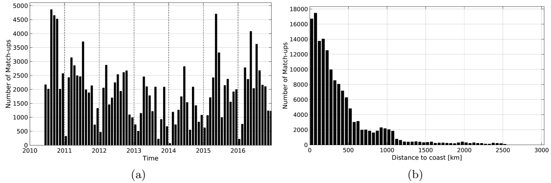
Figure 1: Number of match-ups between TSG-LEGOS-DM and SMOS-L2-DPGS-v662 SSS as a function of time (a) and as function of the distance to coast (b) over the Equatorial Ocean 10N-10S Pi-MEP region and for the full satellite product period.
