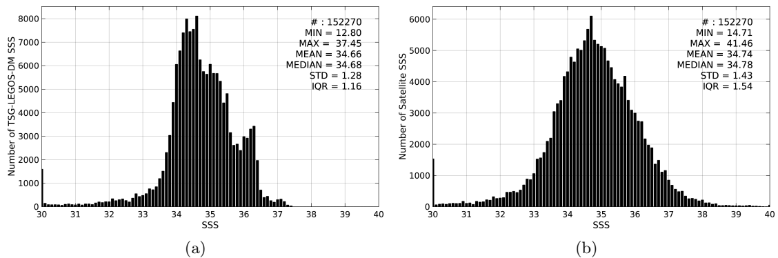
Figure 2: Histograms of SSS from TSG-LEGOS-DM (a) and SMOS-L2-DPGS-v662 (b) considering all match-up pairs per bins of 0.1 over the Equatorial Ocean 10N-10S Pi-MEP region and for the full satellite product period.
