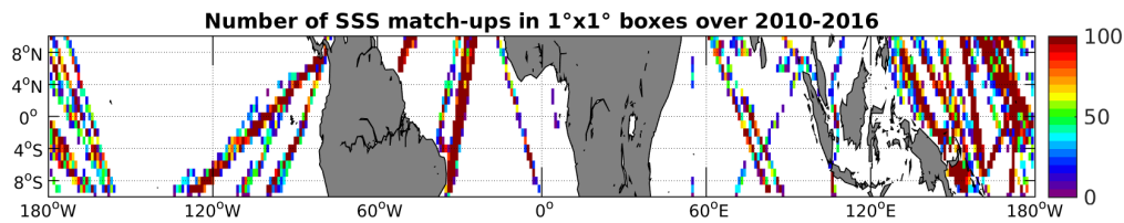
Figure 4: Number of SSS match-ups between TSG-LEGOS-DM SSS and the SMOS-L2-DPGS-v662 SSS product for the Equatorial Ocean 10N-10S Pi-MEP region over 1^\circ \times 1^\circ boxes and for the full satellite product period.
