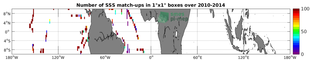
Figure 4: Number of SSS match-ups between TSG (GOSUD-Sailing-ship) SSS and the SMOS SSS L2 v662 (ESA) SSS product for the Equatorial Ocean 10N-10S Pi-MEP region over 1^\circ \times 1^\circ boxes and for the full satellite product period.
