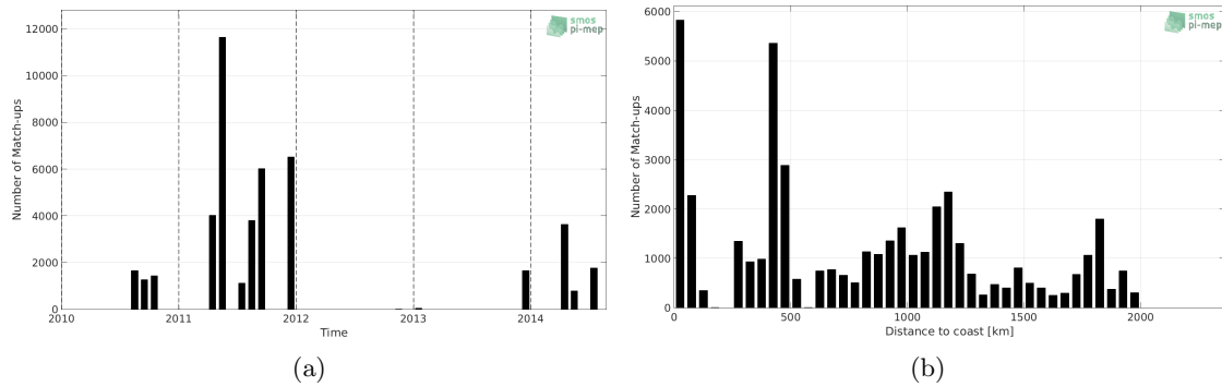
Figure 1: Number of match-ups between TSG (GOSUD-Sailing-ship) and SMOS SSS L2 v662 (ESA) SSS as a function of time (a) and as function of the distance to coast (b) over the Equatorial Ocean 10N-10S Pi-MEP region and for the full satellite product period.
