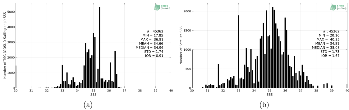
Figure 2: Histograms of SSS from TSG (GOSUD-Sailing-ship) (a) and SMOS SSS L2 v662 (ESA) (b) considering all match-up pairs per bins of 0.1 over the Equatorial Ocean 10N-10S Pi-MEP region and for the full satellite product period.
