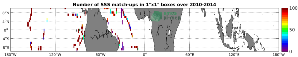
Figure 4: Number of SSS match-ups between TSG (GOSUD-Sailing-ship) SSS and the SMOS SSS L2 v662 (ESA) SSS product for the Equatorial Ocean 10N-10S Pi-MEP region over 1°x1° boxes and for the full satellite product period.
