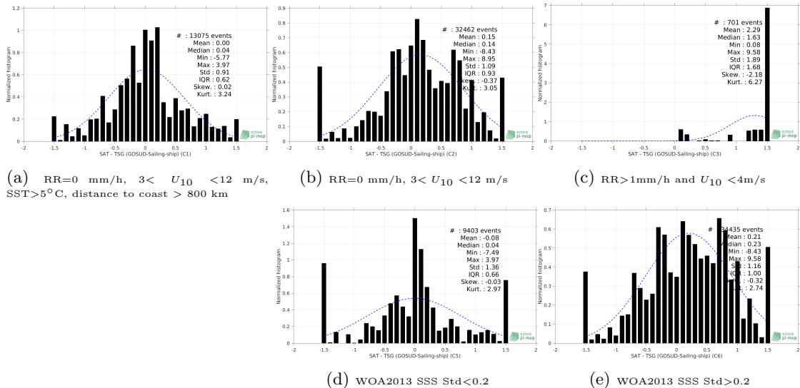
Figure 13: Normalized histogram of ΔSSS (SMOS SSS L2 v662 (ESA) - TSG (GOSUD-Sailing-ship)) for 5 different subdatasets corresponding to: RR=0 mm/h, 3 < U_{10} < 12 m/s, SST>5°C, distance to coast > 800 km (a), RR=0 mm/h, 3 < U_{10} < 12 m/s (b), RR>1mm/h and U_{10} < 4m/s (c), WOA2013 SSS Std<0.2 (d), WOA2013 SSS Std>0.2 (e).
