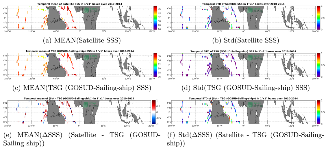
Figure 6: Temporal mean (left) and Std (right) of SSS from SMOS SSS L2 v662 (ESA) (top), TSG (GOSUD-Sailing-ship) (middle), and of \Delta SSS (Satellite - TSG (GOSUD-Sailing-ship)). Only match-up pairs are used to generate these maps.
