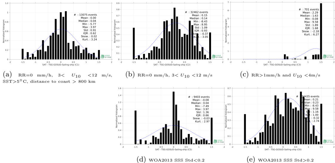
Figure 13: Normalized histogram of ΔSSS (SMOS L2 v662 (ESA) - TSG-GOSUD-Sailing-ship) for 5 different subdatasets corresponding to: RR=0 mm/h, 3 < U 10 < 12 m/s, SST > 5°C, distance to coast > 800 km (a), RR=0 mm/h, 3 < U 10 < 12 m/s (b), RR > 1mm/h and U 10 < 4m/s (c), WOA2013 SSS Std < 0.2 (d), WOA2013 SSS Std > 0.2 (e).
