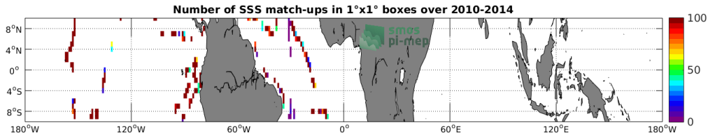
Figure 4: Number of SSS match-ups between TSG-GOSUD-Sailing-ship SSS and the SMOS L2 v662 (ESA) SSS product for the Equatorial Ocean 10N-10S Pi-MEP region over 1°x1° boxes and for the full satellite product period.
