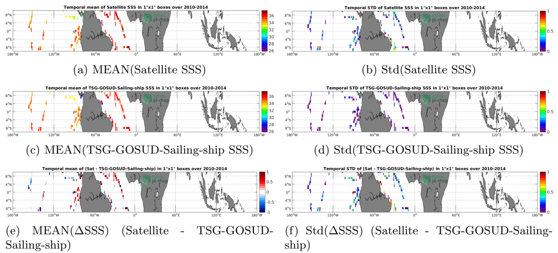
Figure 6: Temporal mean (left) and Std (right) of SSS from SMOS L2 v662 (ESA) (top), TSG-GOSUD-Sailing-ship (middle), and of \Delta SSS (Satellite - TSG-GOSUD-Sailing-ship). Only match-up pairs are used to generate these maps.
