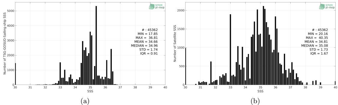
Figure 2: Histograms of SSS from TSG-GOSUD-Sailing-ship (a) and SMOS L2 v662 (ESA) (b) considering all match-up pairs per bins of 0.1 over the Equatorial Ocean 10N-10S Pi-MEP region and for the full satellite product period.
