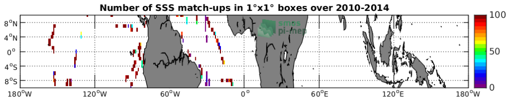
Figure 4: Number of SSS match-ups between TSG-GOSUD-Sailing-ship SSS and the SMOS-L2-DPGS-v662 SSS product for the Equatorial Ocean 10N-10S Pi-MEP region over 1°x1° boxes and for the full satellite product period.
