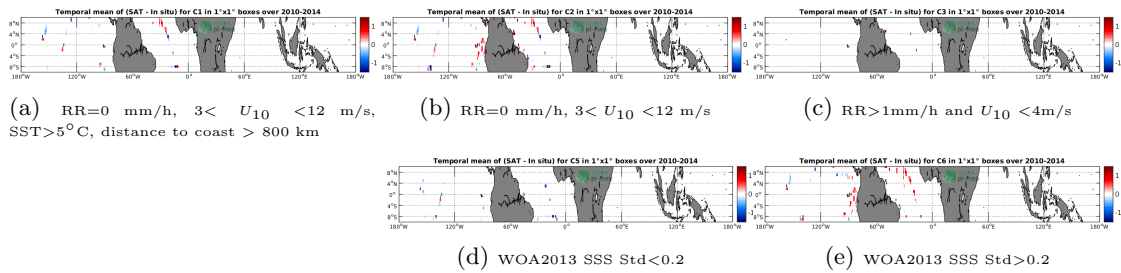
Figure 12: Temporal mean gridded over spatial boxes of size 1^\circ \times 1^\circ of \Delta SSS (SMOS-L2-DPGS-v662 - TSG-GOSUD-Sailing-ship) for 5 different subdatasets corresponding to: RR=0 mm/h, 3 < U_{10} < 12 m/s, SST>5°C, distance to coast > 800 km (a), RR=0 mm/h, 3 < U_{10} < 12 m/s (b), RR>1mm/h and U_{10} < 4 m/s (c), WOA2013 SSS Std<0.2 (d), WOA2013 SSS Std>0.2 (e).
