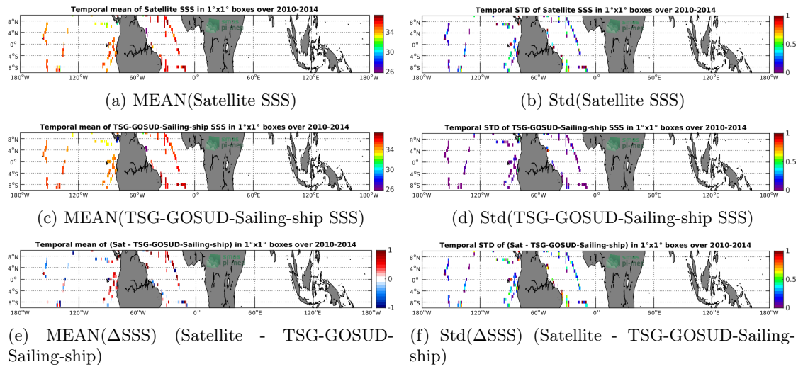
Figure 6: Temporal mean (left) and Std (right) of SSS from SMOS-L2-DPGS-v662 (top), TSG-GOSUD-Sailing-ship (middle), and of \Delta SSS (Satellite - TSG-GOSUD-Sailing-ship). Only match-up pairs are used to generate these maps.
