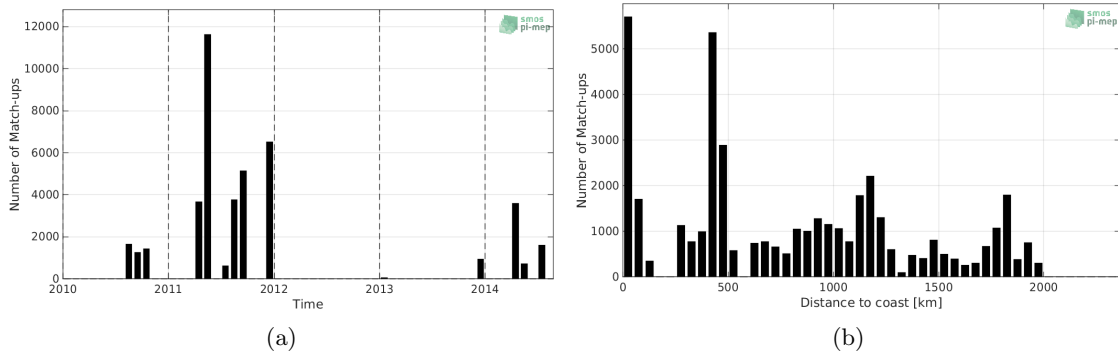
Figure 1: Number of match-ups between TSG-GOSUD-Sailing-ship and SMOS-L2-DPGS-v662 SSS as a function of time (a) and as function of the distance to coast (b) over the Equatorial Ocean 10N-10S Pi-MEP region and for the full satellite product period.
