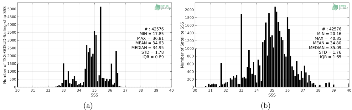
Figure 2: Histograms of SSS from TSG-GOSUD-Sailing-ship (a) and SMOS-L2-DPGS-v662 (b) considering all match-up pairs per bins of 0.1 over the Equatorial Ocean 10N-10S Pi-MEP region and for the full satellite product period.
