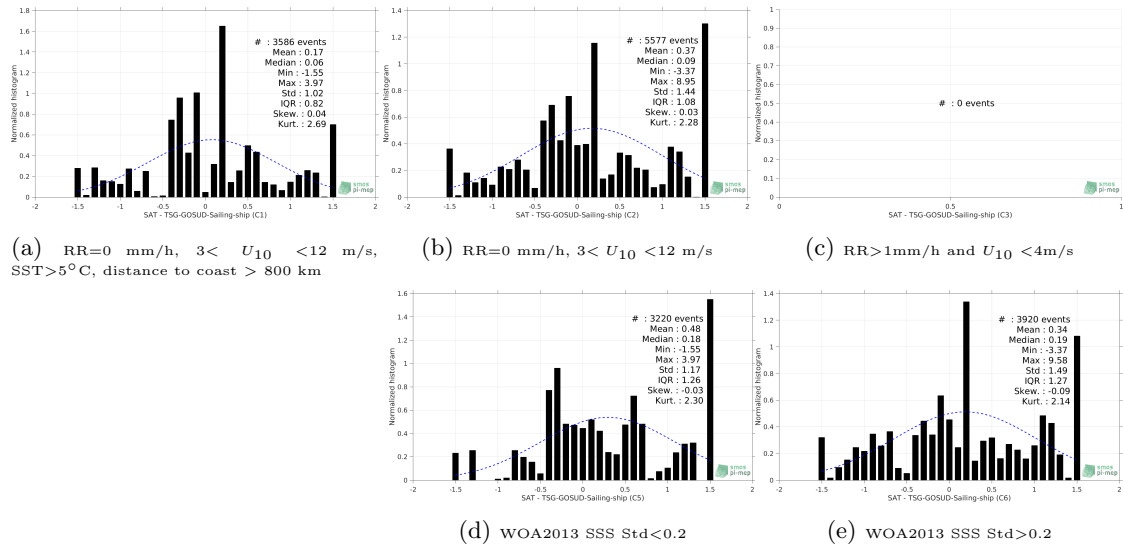
Figure 13: Normalized histogram of \Delta SSS (SMOS-L2-DPGS-v662 - TSG-GOSUD-Sailing-ship) for 5 different subdatasets corresponding to: RR=0 mm/h, 3 < U_{10} < 12 m/s, SST >5^\circ\text{C} , distance to coast > 800 km (a), RR=0 mm/h, 3 < U_{10} < 12 m/s (b), RR >1 mm/h and U_{10} < 4 m/s (c), WOA2013 SSS Std <0.2 (d), WOA2013 SSS Std >0.2 (e).
