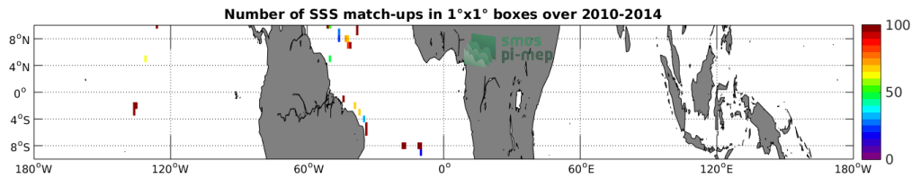
Figure 4: Number of SSS match-ups between TSG-GOSUD-Sailing-ship SSS and the SMOS-L2-DPGS-v662 SSS product for the Equatorial Ocean 10N-10S Pi-MEP region over 1^\circ \times 1^\circ boxes and for the full satellite product period.
