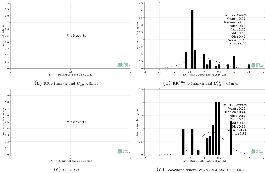
Figure 13: Normalized histogram of \Delta SSS (SMOS-L2-DPGS-v662 - TSG-GOSUD-Sailing-ship) for 6 different subdatasets corresponding to: RR > 1\text{mm/h} and U_{10} < 5\text{m/s} (a), RR^{10d} > 5\text{mm/h} and U_{10}^{10d} < 5\text{m/s} (b), C1 U C2 (c), Locations where WOA2013 SSS STD > 0.2 (d).
