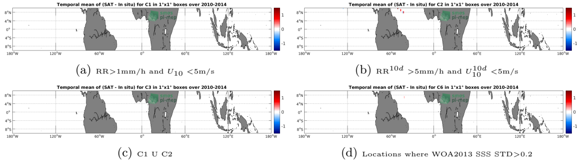
Figure 12: Temporal mean gridded over spatial boxes of size 1^\circ \times 1^\circ of \Delta SSS (SMOS-L2-DPGS-v662 - TSG-GOSUD-Sailing-ship) for 4 different subdatasets corresponding to: RR > 1\text{mm/h} and U_{10} < 5\text{m/s} (a), RR^{10d} > 5\text{mm/h} and U_{10}^{10d} < 5\text{m/s} (b), C1 U C2 (c), Locations where WOA2013 SSS STD > 0.2 (d).
