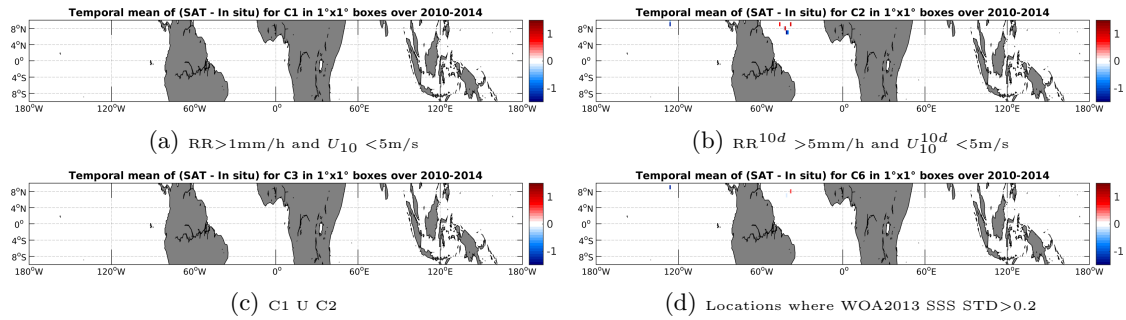
Figure 12: Temporal mean gridded over spatial boxes of size 1^\circ \times 1^\circ of \Delta SSS (SMOS-L2-DPGS-v662 - TSG-GOSUD-Sailing-ship) for 4 different subdatasets corresponding to: RR > 1\text{mm/h} and U_{10} < 5\text{m/s} (a), RR^{10d} > 5\text{mm/h} and U_{10}^{10d} < 5\text{m/s} (b), C1 U C2 (c), Locations where WOA2013 SSS STD > 0.2 (d).
