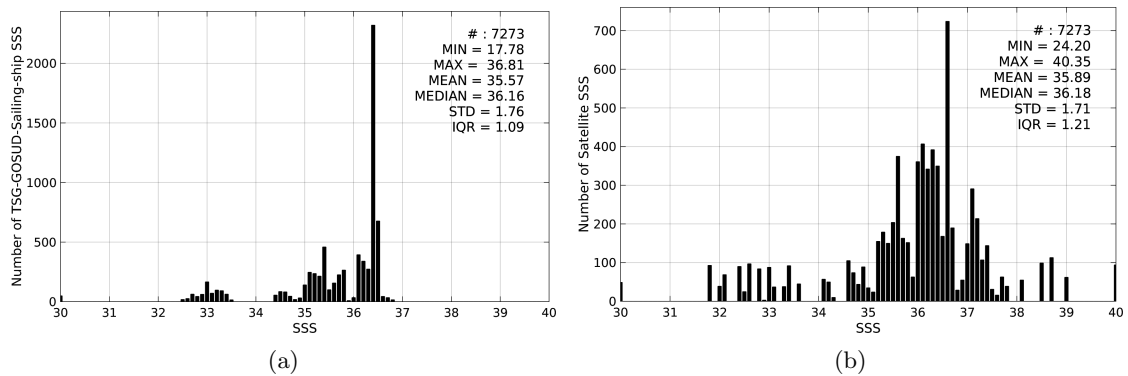
Figure 2: Histograms of SSS from TSG-GOSUD-Sailing-ship (a) and SMOS-L2-DPGS-v662 (b) considering all match-up pairs per bins of 0.1 over the Equatorial Ocean 10N-10S Pi-MEP region and for the full satellite product period.
