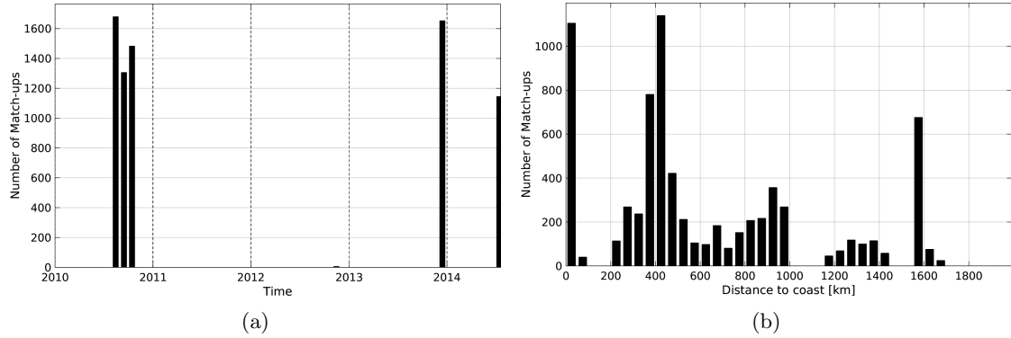
Figure 1: Number of match-ups between TSG-GOSUD-Sailing-ship and SMOS-L2-DPGS-v662 SSS as a function of time (a) and as function of the distance to coast (b) over the Equatorial Ocean 10N-10S Pi-MEP region and for the full satellite product period.
