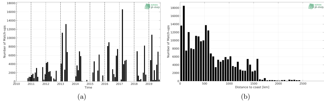
Figure 1: Number of match-ups between TSG (GOSUD-Research-vessel) and SMOS SSS L2 v662 (ESA) SSS as a function of time (a) and as function of the distance to coast (b) over the Equatorial Ocean 10N-10S Pi-MEP region and for the full satellite product period.
