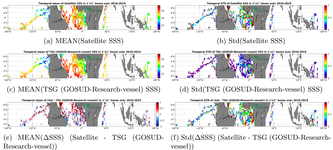
Figure 6: Temporal mean (left) and Std (right) of SSS from SMOS SSS L2 v662 (ESA) (top), TSG (GOSUD-Research-vessel) (middle), and of \Delta SSS (Satellite - TSG (GOSUD-Research-vessel)). Only match-up pairs are used to generate these maps.
