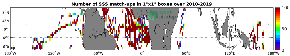
Figure 4: Number of SSS match-ups between TSG (GOSUD-Research-vessel) SSS and the SMOS SSS L2 v662 (ESA) SSS product for the Equatorial Ocean 10N-10S Pi-MEP region over 1^\circ \times 1^\circ boxes and for the full satellite product period.
