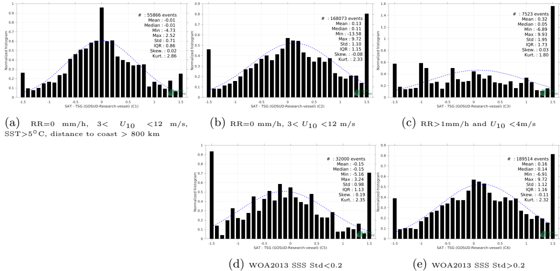
Figure 13: Normalized histogram of \Delta SSS (SMOS SSS L2 v662 (ESA) - TSG (GOSUD-Research-vessel)) for 5 different subdatasets corresponding to: RR=0 mm/h, 3 < U_{10} < 12 m/s, SST> 5^\circ\text{C} , distance to coast > 800 km (a), RR=0 mm/h, 3 < U_{10} < 12 m/s (b), RR>1mm/h and U_{10} < 4\text{m/s} (c), WOA2013 SSS Std<0.2 (d), WOA2013 SSS Std>0.2 (e).
