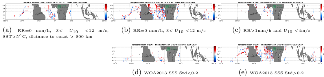
Figure 12: Temporal mean gridded over spatial boxes of size 1^\circ \times 1^\circ of \Delta SSS (SMOS SSS L2 v662 (ESA) - TSG (GOSUD-Research-vessel)) for 5 different subdatasets corresponding to: RR=0 mm/h, 3 < U_{10} < 12 m/s, SST> 5^\circ\text{C} , distance to coast > 800 km (a), RR=0 mm/h, 3 < U_{10} < 12 m/s (b), RR>1mm/h and U_{10} < 4\text{m/s} (c), WOA2013 SSS Std<0.2 (d), WOA2013 SSS Std>0.2 (e).
