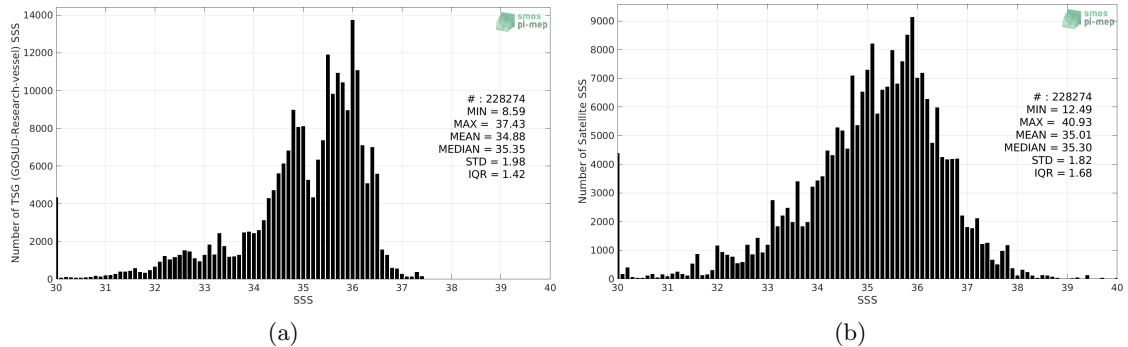
Figure 2: Histograms of SSS from TSG (GOSUD-Research-vessel) (a) and SMOS SSS L2 v662 (ESA) (b) considering all match-up pairs per bins of 0.1 over the Equatorial Ocean 10N-10S Pi-MEP region and for the full satellite product period.
