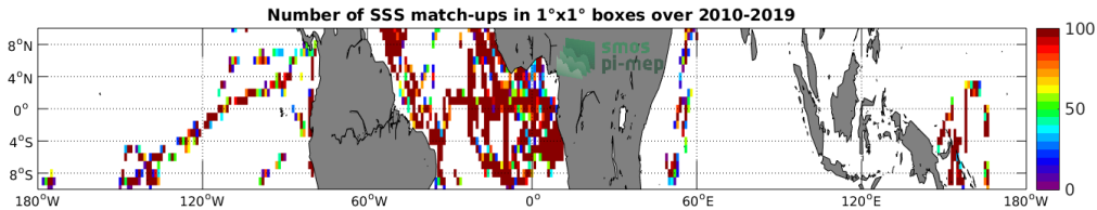
Figure 4: Number of SSS match-ups between TSG (GOSUD-Research-vessel) SSS and the SMOS SSS L2 v662 (ESA) SSS product for the Equatorial Ocean 10N-10S Pi-MEP region over 1°x1° boxes and for the full satellite product period.
