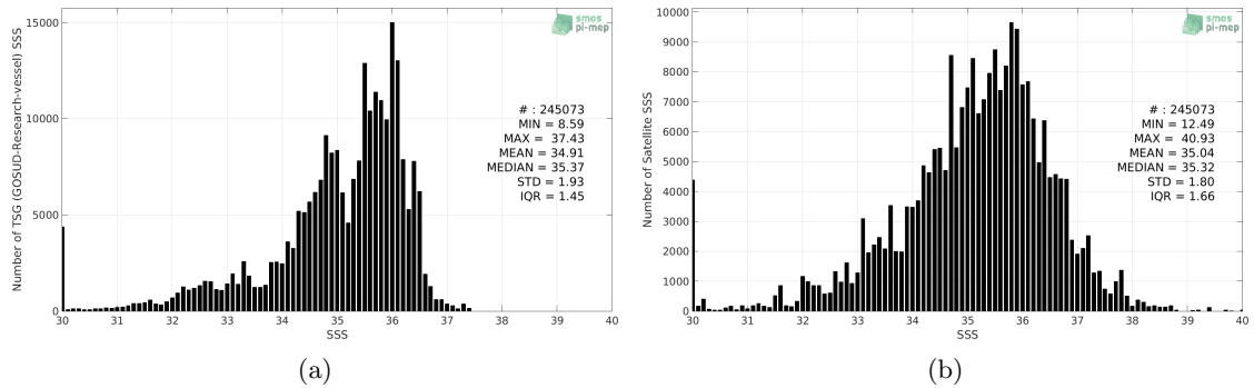
Figure 2: Histograms of SSS from TSG (GOSUD-Research-vessel) (a) and SMOS SSS L2 v662 (ESA) (b) considering all match-up pairs per bins of 0.1 over the Equatorial Ocean 10N-10S Pi-MEP region and for the full satellite product period.
