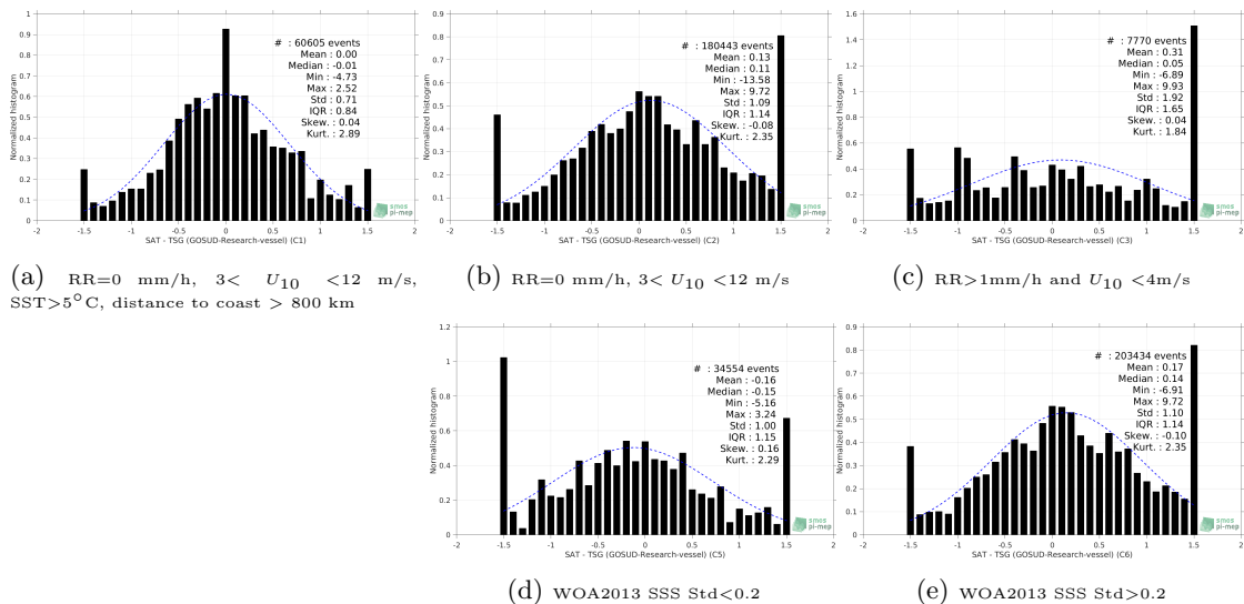
Figure 13: Normalized histogram of ΔSSS (SMOS SSS L2 v662 (ESA) - TSG (GOSUD-Research-vessel)) for 5 different subdatasets corresponding to: RR=0 mm/h, 3 < U_{10} < 12 m/s, SST>5°C, distance to coast > 800 km (a), RR=0 mm/h, 3 < U_{10} < 12 m/s (b), RR>1mm/h and U_{10} < 4m/s (c), WOA2013 SSS Std<0.2 (d), WOA2013 SSS Std>0.2 (e).
