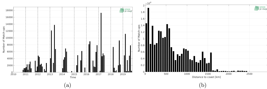
Figure 1: Number of match-ups between TSG (GOSUD-Research-vessel) and SMOS SSS L2 v662 (ESA) SSS as a function of time (a) and as function of the distance to coast (b) over the Equatorial Ocean 10N-10S Pi-MEP region and for the full satellite product period.
