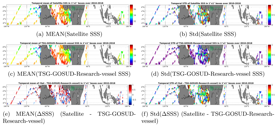
Figure 6: Temporal mean (left) and Std (right) of SSS from SMOS L2 v662 (ESA) (top), TSG-GOSUD-Research-vessel (middle), and of \Delta SSS (Satellite - TSG-GOSUD-Research-vessel). Only match-up pairs are used to generate these maps.
