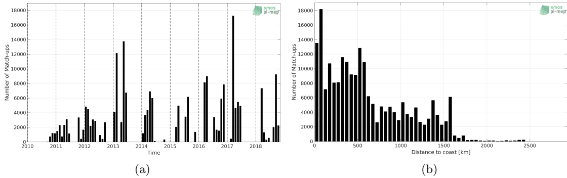
Figure 1: Number of match-ups between TSG-GOSUD-Research-vessel and SMOS L2 v662 (ESA) SSS as a function of time (a) and as function of the distance to coast (b) over the Equatorial Ocean 10N-10S Pi-MEP region and for the full satellite product period.
