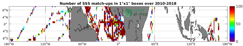
Figure 4: Number of SSS match-ups between TSG-GOSUD-Research-vessel SSS and the SMOS L2 v662 (ESA) SSS product for the Equatorial Ocean 10N-10S Pi-MEP region over 1°x1° boxes and for the full satellite product period.
