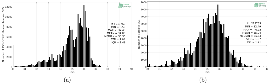
Figure 2: Histograms of SSS from TSG-GOSUD-Research-vessel (a) and SMOS L2 v662 (ESA) (b) considering all match-up pairs per bins of 0.1 over the Equatorial Ocean 10N-10S Pi-MEP region and for the full satellite product period.
