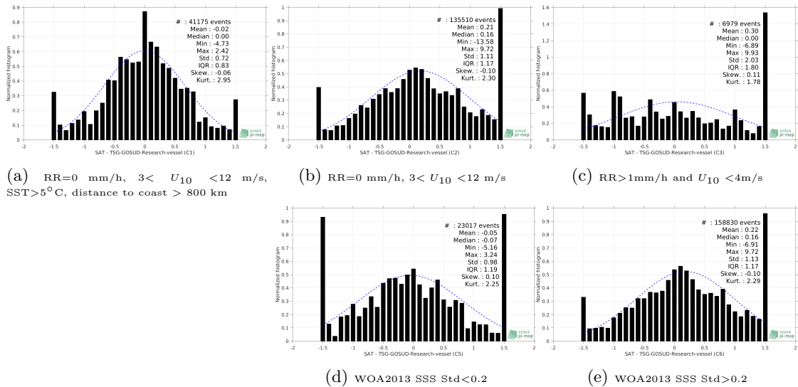
Figure 13: Normalized histogram of \Delta SSS (SMOS-L2-DPGS-v662 - TSG-GOSUD-Research-vessel) for 5 different subdatasets corresponding to: RR=0 mm/h, 3 < U_{10} < 12 m/s, SST >5^\circ\text{C} , distance to coast > 800 km (a), RR=0 mm/h, 3 < U_{10} < 12 m/s (b), RR >1 mm/h and U_{10} < 4 m/s (c), WOA2013 SSS Std <0.2 (d), WOA2013 SSS Std >0.2 (e).
