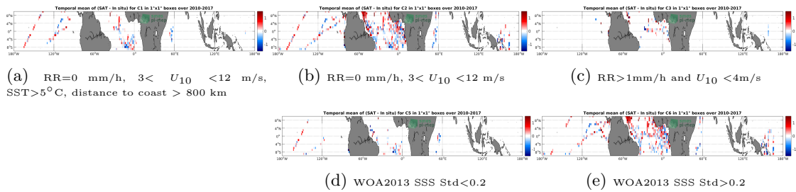
Figure 12: Temporal mean gridded over spatial boxes of size 1^\circ \times 1^\circ of \Delta SSS (SMOS-L2-DPGS-v662 - TSG-GOSUD-Research-vessel) for 5 different subdatasets corresponding to:RR=0 mm/h, 3 < U_{10} < 12 m/s, SST >5^\circ\text{C} , distance to coast > 800 km (a), RR=0 mm/h, 3 < U_{10} < 12 m/s (b), RR >1 mm/h and U_{10} < 4 m/s (c), WOA2013 SSS Std <0.2 (d), WOA2013 SSS Std >0.2 (e).
