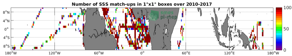
Figure 4: Number of SSS match-ups between TSG-GOSUD-Research-vessel SSS and the SMOS-L2-DPGS-v662 SSS product for the Equatorial Ocean 10N-10S Pi-MEP region over 1°x1° boxes and for the full satellite product period.
