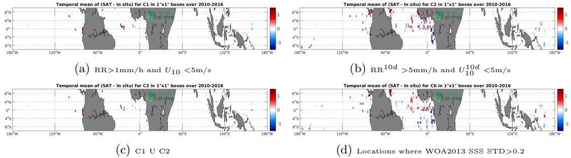
Figure 12: Temporal mean gridded over spatial boxes of size 1^\circ \times 1^\circ of \Delta SSS (SMOS-L2-DPGS-v662 - TSG-GOSUD-Research-vessel) for 4 different subdatasets corresponding to: RR > 1\text{mm/h} and U_{10} < 5\text{m/s} (a), RR^{10d} > 5\text{mm/h} and U_{10}^{10d} < 5\text{m/s} (b), C1 U C2 (c), Locations where WOA2013 SSS STD > 0.2 (d).
