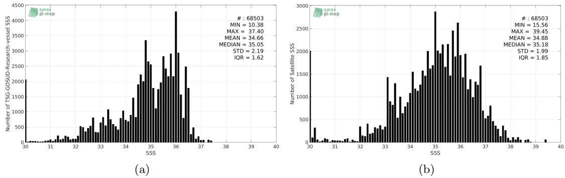
Figure 2: Histograms of SSS from TSG-GOSUD-Research-vessel (a) and SMOS-L2-DPGS-v662 (b) considering all match-up pairs per bins of 0.1 over the Equatorial Ocean 10N-10S Pi-MEP region and for the full satellite product period.
