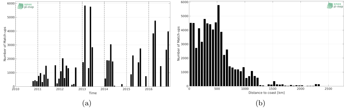
Figure 1: Number of match-ups between TSG-GOSUD-Research-vessel and SMOS-L2-DPGS-v662 SSS as a function of time (a) and as function of the distance to coast (b) over the Equatorial Ocean 10N-10S Pi-MEP region and for the full satellite product period.
