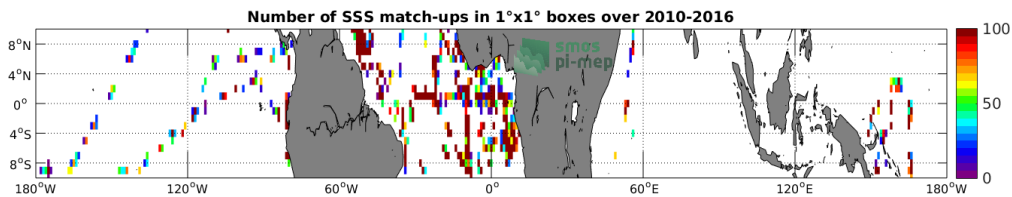
Figure 4: Number of SSS match-ups between TSG-GOSUD-Research-vessel SSS and the SMOS-L2-DPGS-v662 SSS product for the Equatorial Ocean 10N-10S Pi-MEP region over 1^\circ \times 1^\circ boxes and for the full satellite product period.
