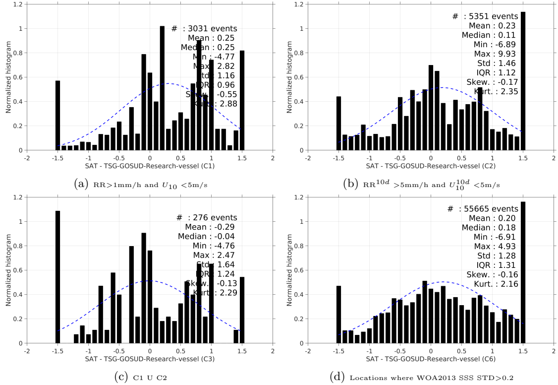
Figure 13: Normalized histogram of \Delta SSS (SMOS-L2-DPGS-v662 - TSG-GOSUD-Research-vessel) for 6 different subdatasets corresponding to: RR > 1\text{mm/h} and U_{10} < 5\text{m/s} (a), RR^{10d} > 5\text{mm/h} and U_{10}^{10d} < 5\text{m/s} (b), C1 \cup C2 (c), Locations where WOA2013 SSS STD > 0.2 (d).
