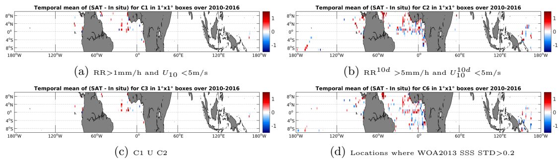
Figure 12: Temporal mean gridded over spatial boxes of size 1^\circ \times 1^\circ of \Delta SSS (SMOS-L2-DPGS-v662 - TSG-GOSUD-Research-vessel) for 4 different subdatasets corresponding to:RR > 1 mm/h and U_{10} < 5 m/s (a), RR 10d > 5 mm/h and U_{10}^{10d} < 5 m/s (b), C1 U C2 (c),Locations where WOA2013 SSS STD > 0.2 (d).
