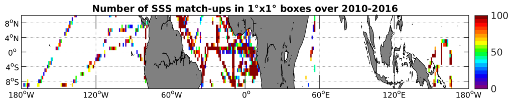
Figure 4: Number of SSS match-ups between TSG-GOSUD-Research-vessel SSS and the SMOS-L2-DPGS-v662 SSS product for the Equatorial Ocean 10N-10S Pi-MEP region over 1°x1° boxes and for the full satellite product period.
