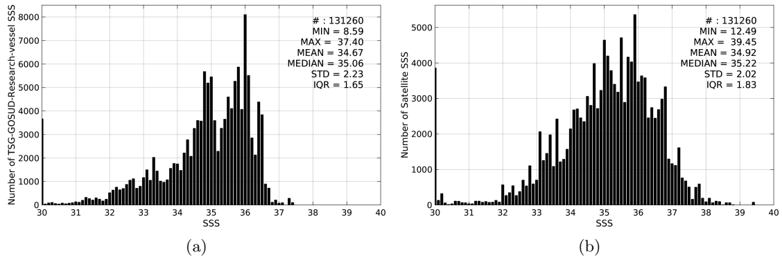
Figure 2: Histograms of SSS from TSG-GOSUD-Research-vessel (a) and SMOS-L2-DPGS-v662 (b) considering all match-up pairs per bins of 0.1 over the Equatorial Ocean 10N-10S Pi-MEP region and for the full satellite product period.
