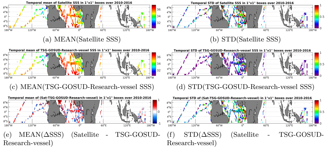
Figure 6: Temporal mean (left) and STD (right) of SSS from SMOS-L2-DPGS-v662 (top), TSG-GOSUD-Research-vessel (middle), and of \Delta SSS (Satellite - TSG-GOSUD-Research-vessel). Only match-up pairs are used to generate these maps.
