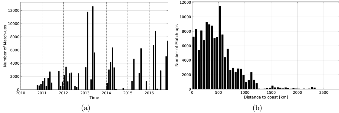
Figure 1: Number of match-ups between TSG-GOSUD-Research-vessel and SMOS-L2-DPGS-v662 SSS as a function of time (a) and as function of the distance to coast (b) over the Equatorial Ocean 10N-10S Pi-MEP region and for the full satellite product period.
