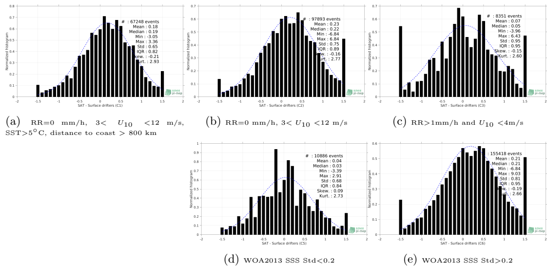
Figure 12: Normalized histogram of \Delta SSS (SMOS SSS L2 v662 (ESA) - Surface drifters) for 5 different subdatasets corresponding to: RR=0 mm/h, 3 < U_{10} < 12 m/s, SST>5°C, distance to coast > 800 km (a), RR=0 mm/h, 3 < U_{10} < 12 m/s (b), RR>1mm/h and U_{10} < 4m/s (c), WOA2013 SSS Std<0.2 (d), WOA2013 SSS Std>0.2 (e).
