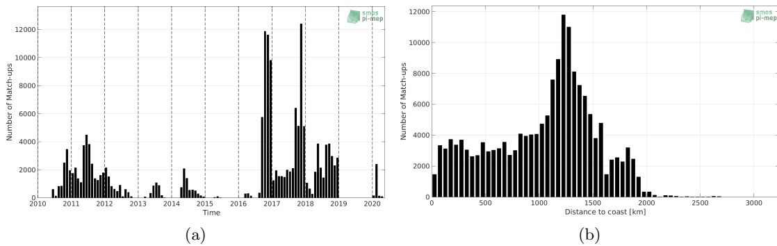
Figure 1: Number of match-ups between Surface drifters and SMOS SSS L2 v662 (ESA) SSS as a function of time (a) and as function of the distance to coast (b) over the Equatorial Ocean 10N-10S Pi-MEP region and for the full satellite product period.
