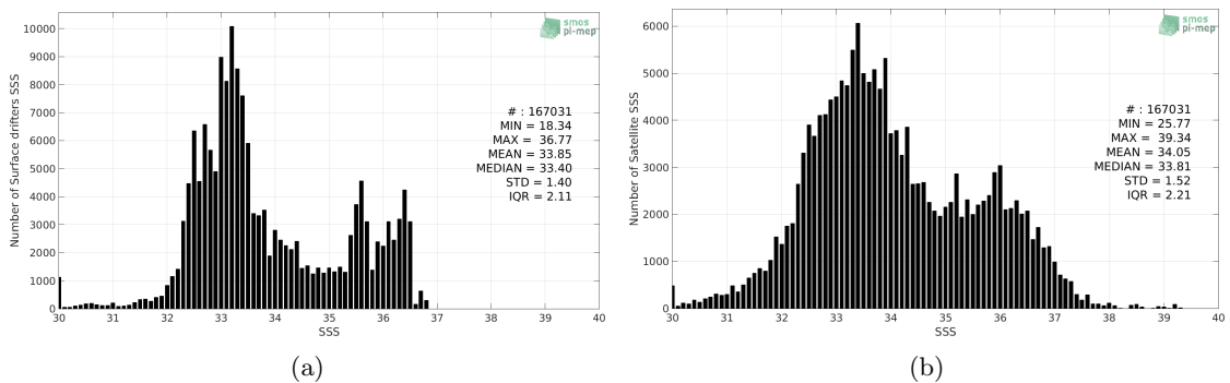
Figure 2: Histograms of SSS from Surface drifters (a) and SMOS SSS L2 v662 (ESA) (b) considering all match-up pairs per bins of 0.1 over the Equatorial Ocean 10N-10S Pi-MEP region and for the full satellite product period.
