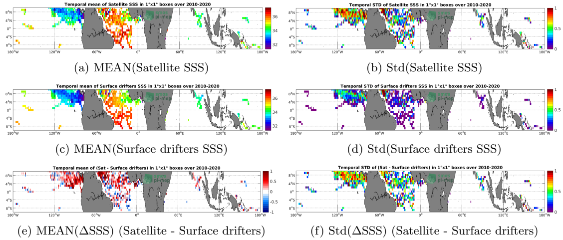
Figure 5: Temporal mean (left) and Std (right) of SSS from SMOS SSS L2 v662 (ESA) (top), Surface drifters (middle), and of \Delta SSS (Satellite - Surface drifters). Only match-up pairs are used to generate these maps.
