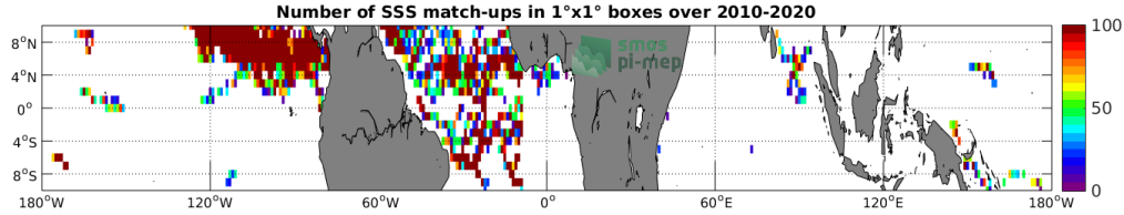
Figure 3: Number of SSS match-ups between Surface drifters SSS and the SMOS SSS L2 v662 (ESA) SSS product for the Equatorial Ocean 10N-10S Pi-MEP region over 1^\circ \times 1^\circ boxes and for the full satellite product period.
