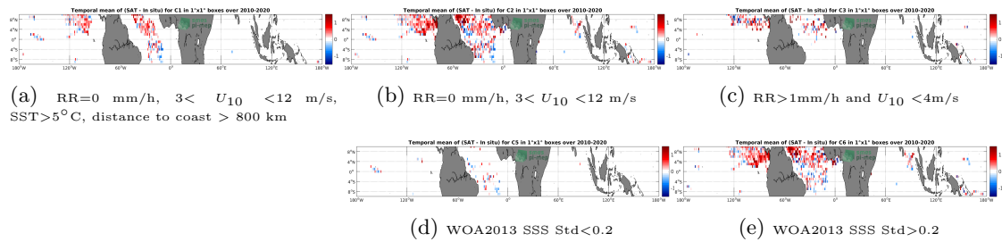
Figure 11: Temporal mean gridded over spatial boxes of size 1°x1° of \Delta SSS (SMOS SSS L2 v662 (ESA) - Surface drifters) for 5 different subdatasets corresponding to:RR=0 mm/h, 3 < U_{10} < 12 m/s, SST>5°C, distance to coast > 800 km (a), RR=0 mm/h, 3 < U_{10} < 12 m/s (b), RR>1mm/h and U_{10} < 4m/s (c), WOA2013 SSS Std<0.2 (d), WOA2013 SSS Std>0.2 (e).
