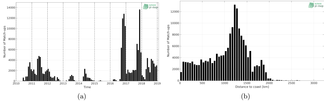
Figure 1: Number of match-ups between Surface drifters and SMOS L2 v662 (ESA) SSS as a function of time (a) and as function of the distance to coast (b) over the Equatorial Ocean 10N-10S Pi-MEP region and for the full satellite product period.
