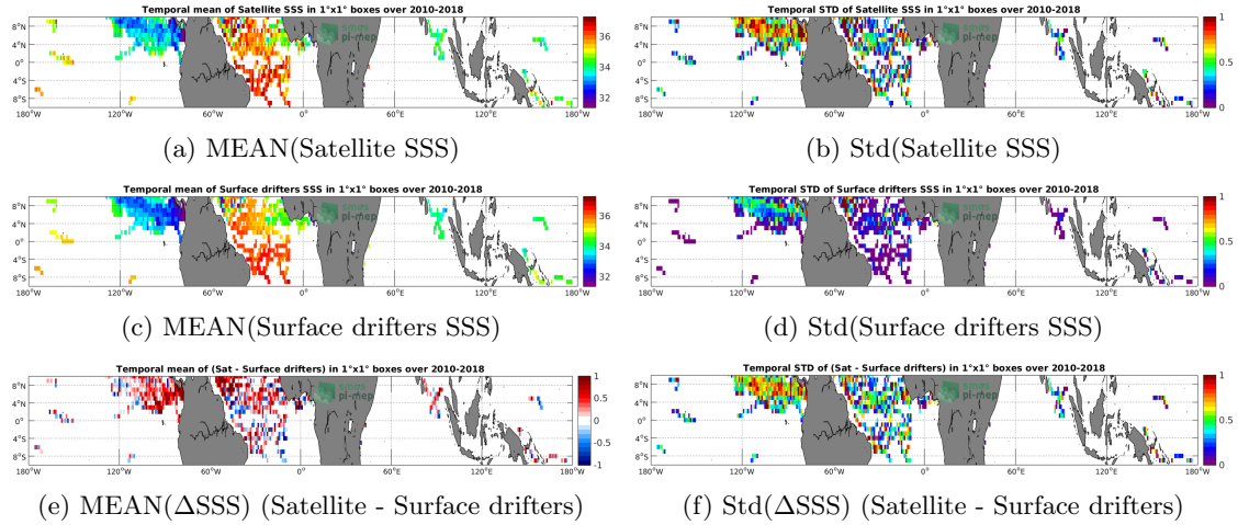
Figure 5: Temporal mean (left) and Std (right) of SSS from SMOS L2 v662 (ESA) (top), Surface drifters (middle), and of \Delta SSS (Satellite - Surface drifters). Only match-up pairs are used to generate these maps.
