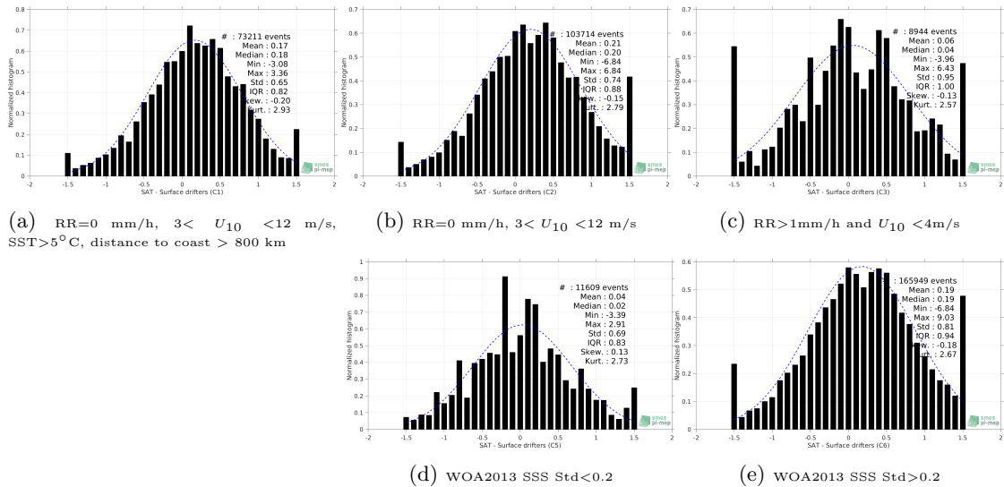
Figure 12: Normalized histogram of ΔSSS (SMOS L2 v662 (ESA) - Surface drifters) for 5 different subdatasets corresponding to: RR=0 mm/h, 3 < U 10 < 12 m/s, SST>5°C, distance to coast > 800 km (a), RR=0 mm/h, 3 < U 10 < 12 m/s (b), RR>1mm/h and U 10 <4m/s (c), WOA2013 SSS Std<0.2 (d), WOA2013 SSS Std>0.2 (e).
