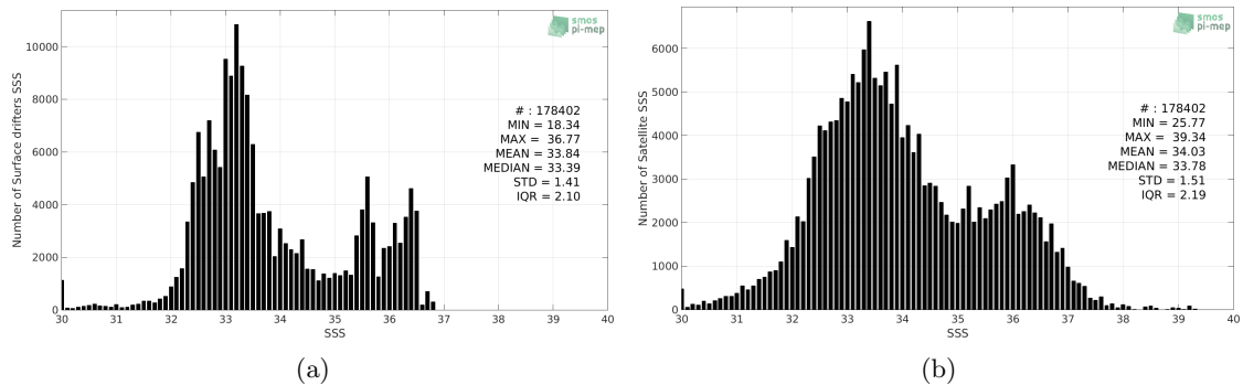
Figure 2: Histograms of SSS from Surface drifters (a) and SMOS L2 v662 (ESA) (b) considering all match-up pairs per bins of 0.1 over the Equatorial Ocean 10N-10S Pi-MEP region and for the full satellite product period.
