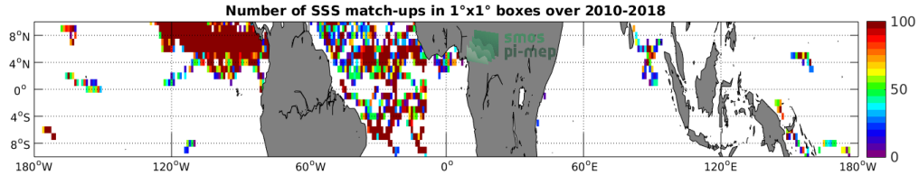
Figure 3: Number of SSS match-ups between Surface drifters SSS and the SMOS L2 v662 (ESA) SSS product for the Equatorial Ocean 10N-10S Pi-MEP region over 1^\circ \times 1^\circ boxes and for the full satellite product period.
