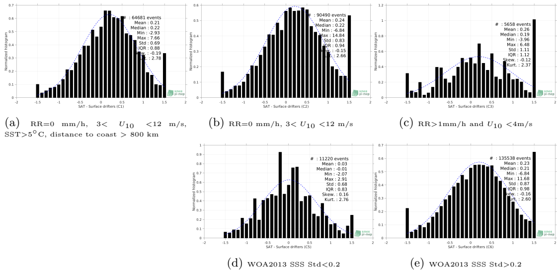
Figure 12: Normalized histogram of \Delta SSS (SMOS-L2-DPGS-v662 - Surface drifters) for 5 different subdatasets corresponding to: RR=0 mm/h, 3 < U_{10} < 12 m/s, SST >5^\circ\text{C} , distance to coast > 800 km (a), RR=0 mm/h, 3 < U_{10} < 12 m/s (b), RR >1 mm/h and U_{10} < 4 m/s (c), WOA2013 SSS Std <0.2 (d), WOA2013 SSS Std >0.2 (e).
