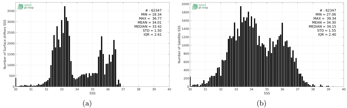
Figure 2: Histograms of SSS from Surface drifters (a) and SMOS-L2-DPGS-v662 (b) considering all match-up pairs per bins of 0.1 over the Equatorial Ocean 10N-10S Pi-MEP region and for the full satellite product period.
