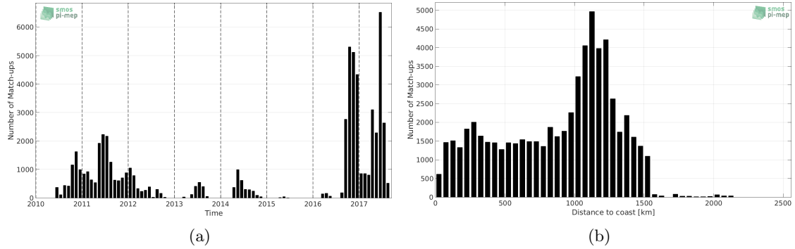
Figure 1: Number of match-ups between Surface drifters and SMOS-L2-DPGS-v662 SSS as a function of time (a) and as function of the distance to coast (b) over the Equatorial Ocean 10N-10S Pi-MEP region and for the full satellite product period.
