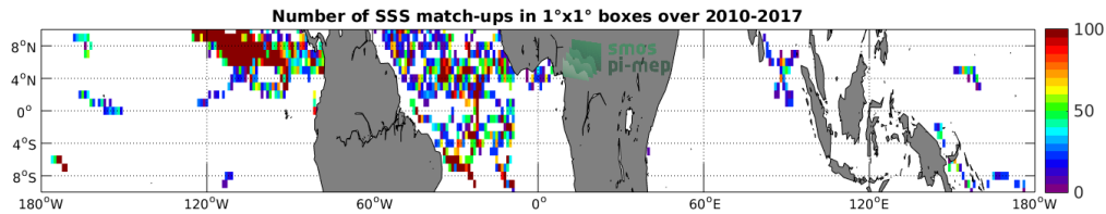
Figure 3: Number of SSS match-ups between Surface drifters SSS and the SMOS-L2-DPGS-v662 SSS product for the Equatorial Ocean 10N-10S Pi-MEP region over 1^\circ \times 1^\circ boxes and for the full satellite product period.
