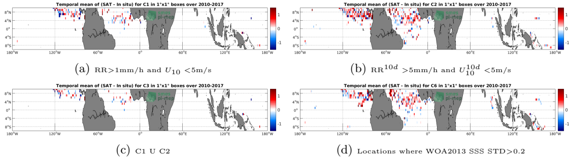
Figure 11: Temporal mean gridded over spatial boxes of size 1^\circ \times 1^\circ of \Delta SSS (SMOS-L2-DPGS-v662 - Surface drifters) for 4 different subdatasets corresponding to: RR > 1\text{mm/h} and U_{10} < 5\text{m/s} (a), RR^{10d} > 5\text{mm/h} and U_{10}^{10d} < 5\text{m/s} (b), C1 U C2 (c), Locations where WOA2013 SSS STD > 0.2 (d).
