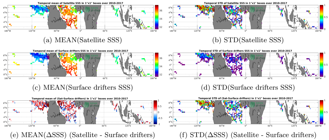
Figure 5: Temporal mean (left) and STD (right) of SSS from SMOS-L2-DPGS-v662 (top), Surface drifters (middle), and of \Delta SSS (Satellite - Surface drifters). Only match-up pairs are used to generate these maps.
