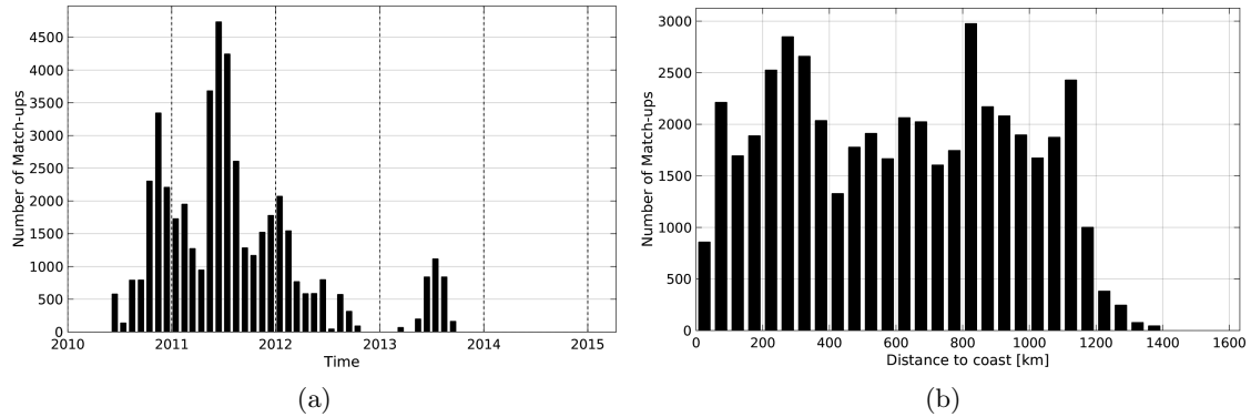
Figure 1: Number of match-ups between Surface drifters and SMOS-L2-DPGS-v662 SSS as a function of time (a) and as function of the distance to coast (b) over the Equatorial Ocean 10N-10S Pi-MEP region and for the full satellite product period.
