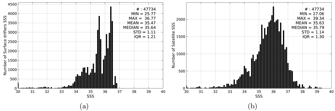
Figure 2: Histograms of SSS from Surface drifters (a) and SMOS-L2-DPGS-v662 (b) considering all match-up pairs per bins of 0.1 over the Equatorial Ocean 10N-10S Pi-MEP region and for the full satellite product period.
