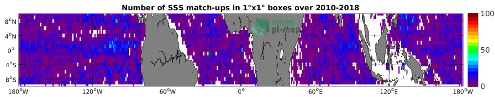
Figure 4: Number of SSS match-ups between Argo SSS and the SMOS-L2-DPGS-v662 SSS product for the Equatorial Ocean 10N-10S Pi-MEP region over 1°x1° boxes and for the full satellite product period.
