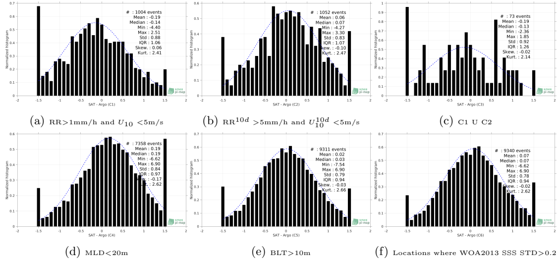
Figure 13: Normalized histogram of \Delta\text{SSS} (SMOS-L2-DPGS-v662 - Argo) for 6 different subdatasets corresponding to: \text{RR} > 1\text{mm/h} and U_{10} < 5\text{m/s} (a), \text{RR}^{10d} > 5\text{mm/h} and U_{10}^{10d} < 5\text{m/s} (b), C1 U C2 (c), \text{MLD} < 20\text{m} (d), \text{BLT} > 10\text{m} (e), Locations where WOA2013 SSS \text{STD} > 0.2 (f).
