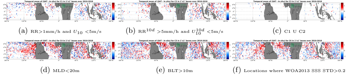
Figure 12: Temporal mean gridded over spatial boxes of size 1^\circ \times 1^\circ of \Delta\text{SSS} (SMOS-L2-DPGS-v662 - Argo) for 6 different subdatasets corresponding to: \text{RR} > 1\text{mm/h} and U_{10} < 5\text{m/s} (a), \text{RR}^{10d} > 5\text{mm/h} and U_{10}^{10d} < 5\text{m/s} (b), C1 U C2 (c), \text{MLD} < 20\text{m} (d), \text{BLT} > 10\text{m} (e), Locations where WOA2013 SSS \text{STD} > 0.2 (f).
