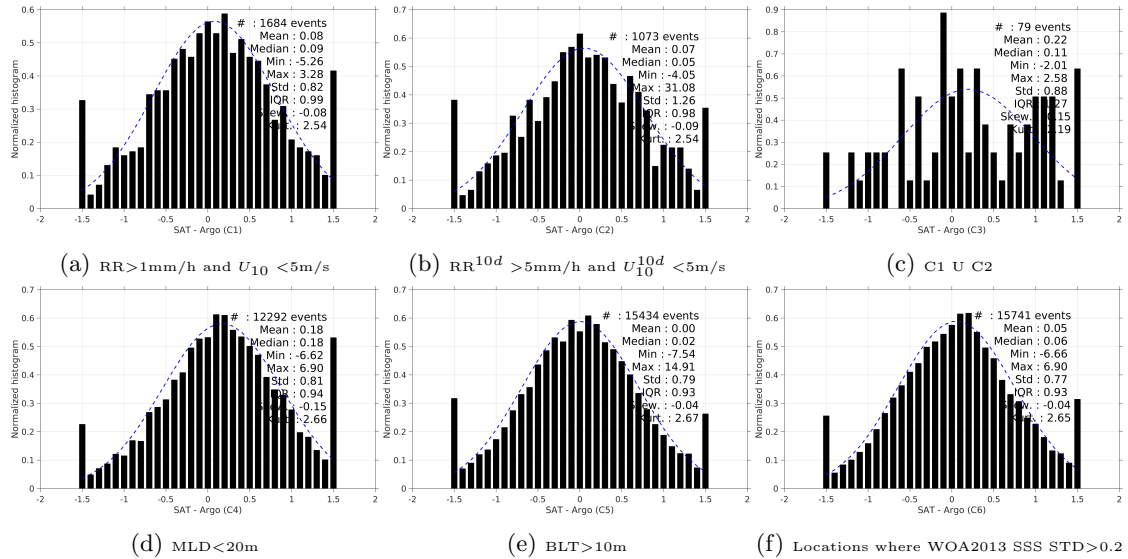
Figure 13: Normalized histogram of \Delta\text{SSS} (SMOS-L2-DPGS-v662 - Argo) for 6 different subdatasets corresponding to: \text{RR} > 1\text{mm/h} and U_{10} < 5\text{m/s} (a), \text{RR}^{10d} > 5\text{mm/h} and U_{10}^{10d} < 5\text{m/s} (b), C1 U C2 (c), \text{MLD} < 20\text{m} (d), \text{BLT} > 10\text{m} (e), Locations where WOA2013 SSS \text{STD} > 0.2 (f).
