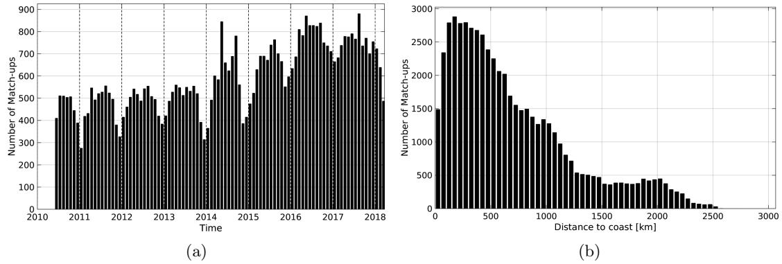
Figure 1: Number of match-ups between Argo and SMOS-L2-DPGS-v662 SSS as a function of time (a) and as function of the distance to coast (b) over the Equatorial Ocean 10N-10S Pi-MEP region and for the full satellite product period.
