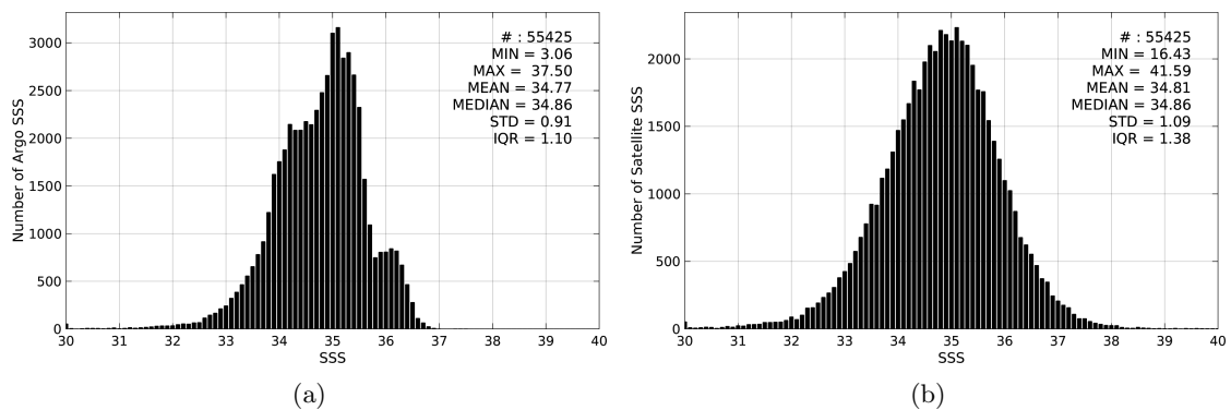
Figure 2: Histograms of SSS from Argo (a) and SMOS-L2-DPGS-v662 (b) considering all match-up pairs per bins of 0.1 over the Equatorial Ocean 10N-10S Pi-MEP region and for the full satellite product period.
