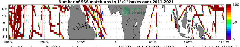
Figure 4: Number of SSS match-ups between TSG (SAMOS) SSS and the SMAP SSS L4 OI v1 - 7 Days (IPRC) SSS product for the Equatorial Ocean 10N-10S Pi-MEP region over 1^\circ \times 1^\circ boxes and for the full satellite product period.
