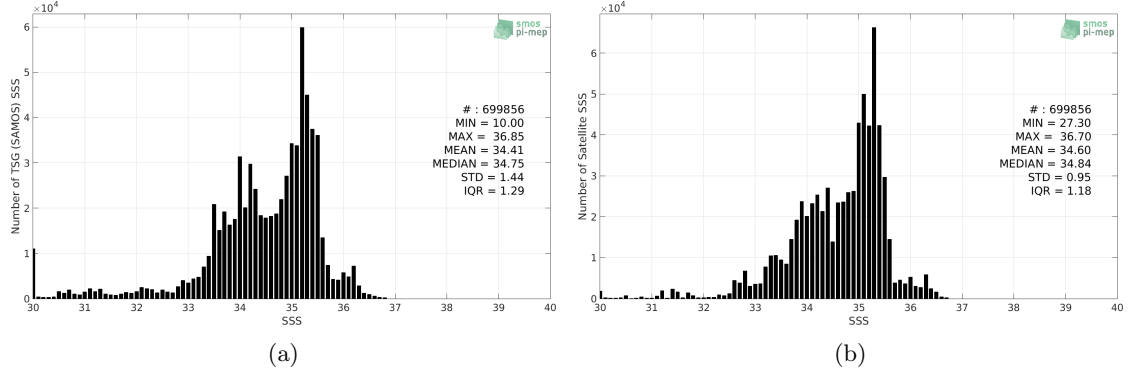
Figure 2: Histograms of SSS from TSG (SAMOS) (a) and SMAP SSS L4 OI v1 - 7 Days (IPRC) (b) considering all match-up pairs per bins of 0.1 over the Equatorial Ocean 10N-10S Pi-MEP region and for the full satellite product period.
