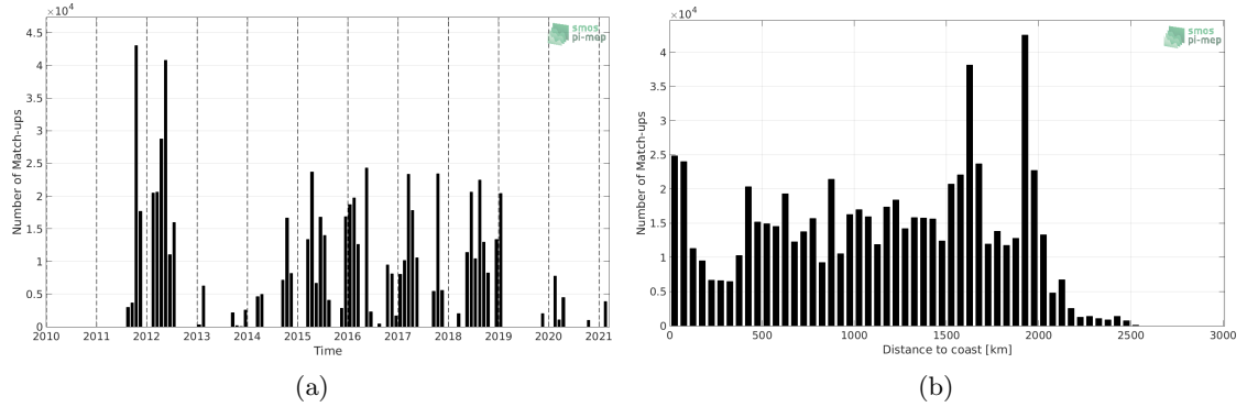
Figure 1: Number of match-ups between TSG (SAMOS) and SMAP SSS L4 OI v1 - 7 Days (IPRC) SSS as a function of time (a) and as function of the distance to coast (b) over the Equatorial Ocean 10N-10S Pi-MEP region and for the full satellite product period.
