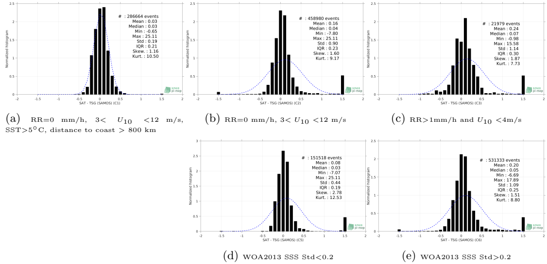
Figure 13: Normalized histogram of \Delta SSS (SMAP SSS L4 OI v1 - 7 Days (IPRC) - TSG (SAMOS)) for 5 different subdatasets corresponding to: RR=0 mm/h, 3 < U_{10} < 12 m/s, SST > 5^\circ\text{C} , distance to coast > 800 km (a), RR=0 mm/h, 3 < U_{10} < 12 m/s (b), RR > 1 mm/h and U_{10} < 4 m/s (c), WOA2013 SSS Std < 0.2 (d), WOA2013 SSS Std > 0.2 (e).
