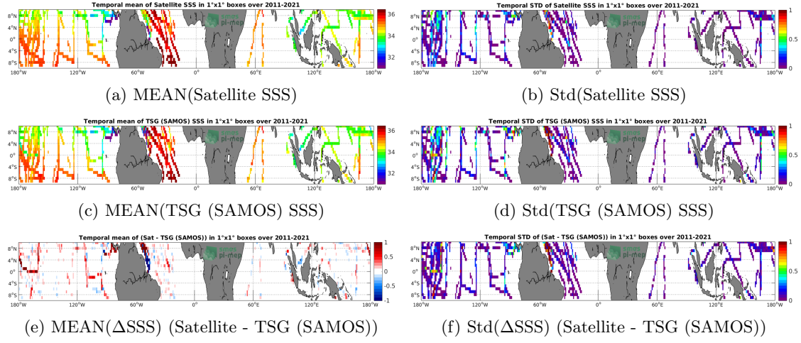
Figure 6: Temporal mean (left) and Std (right) of SSS from SMAP SSS L4 OI v1 - 7 Days (IPRC) (top), TSG (SAMOS) (middle), and of \Delta SSS (Satellite - TSG (SAMOS)). Only match-up pairs are used to generate these maps.
