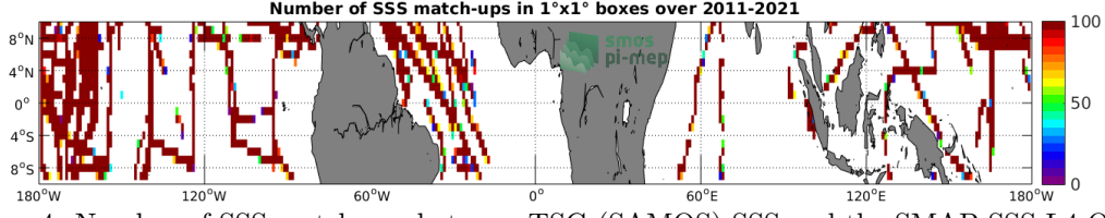
Figure 4: Number of SSS match-ups between TSG (SAMOS) SSS and the SMAP SSS L4 OI v1 - 7day (IPRC) SSS product for the Equatorial Ocean 10N-10S Pi-MEP region over 1^\circ \times 1^\circ boxes and for the full satellite product period.
