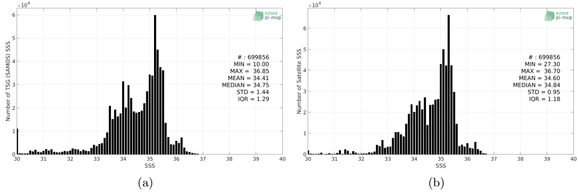
Figure 2: Histograms of SSS from TSG (SAMOS) (a) and SMAP SSS L4 OI v1 - 7day (IPRC) (b) considering all match-up pairs per bins of 0.1 over the Equatorial Ocean 10N-10S Pi-MEP region and for the full satellite product period.
