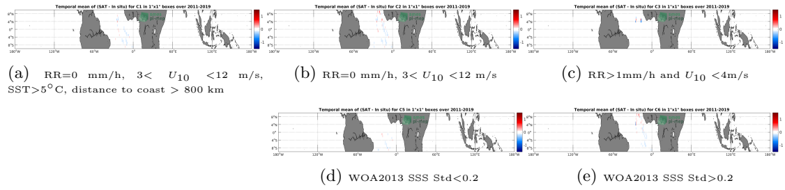
Figure 12: Temporal mean gridded over spatial boxes of size 1^\circ \times 1^\circ of \Delta SSS (SMAP SSS L4 OI v1 - 7day (IPRC) - TSG (Polarstern)) for 5 different subdatasets corresponding to: RR=0 mm/h, 3 < U_{10} < 12 m/s, SST > 5^\circ C , distance to coast > 800 km (a), RR=0 mm/h, 3 < U_{10} < 12 m/s (b), RR > 1 mm/h and U_{10} < 4 m/s (c), WOA2013 SSS Std < 0.2 (d), WOA2013 SSS Std > 0.2 (e).
