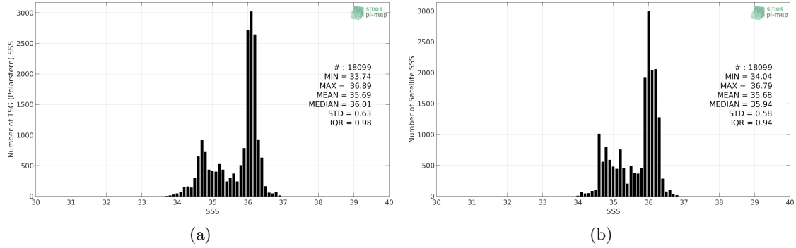
Figure 2: Histograms of SSS from TSG (Polarstern) (a) and SMAP SSS L4 OI v1 - 7day (IPRC) (b) considering all match-up pairs per bins of 0.1 over the Equatorial Ocean 10N-10S Pi-MEP region and for the full satellite product period.
