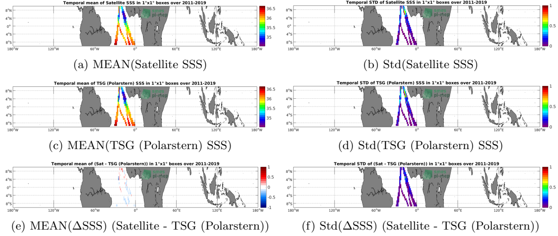
Figure 6: Temporal mean (left) and Std (right) of SSS from SMAP SSS L4 OI v1 - 7day (IPRC) (top), TSG (Polarstern) (middle), and of \Delta SSS (Satellite - TSG (Polarstern)). Only match-up pairs are used to generate these maps.
