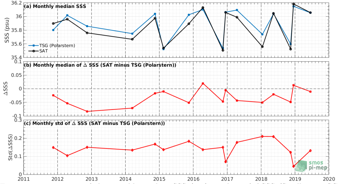
Figure 7: Time series of the monthly median SSS (top), median of \Delta\text{SSS} (Satellite - TSG (Polarstern)) and Std of \Delta\text{SSS} (Satellite - TSG (Polarstern)) over the Equatorial Ocean 10N-10S Pi-MEP region considering all match-ups collected by the Pi-MEP.
