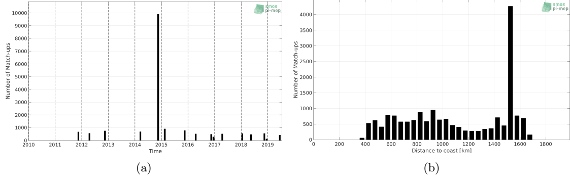
Figure 1: Number of match-ups between TSG (Polarstern) and SMAP SSS L4 OI v1 - 7day (IPRC) SSS as a function of time (a) and as function of the distance to coast (b) over the Equatorial Ocean 10N-10S Pi-MEP region and for the full satellite product period.
