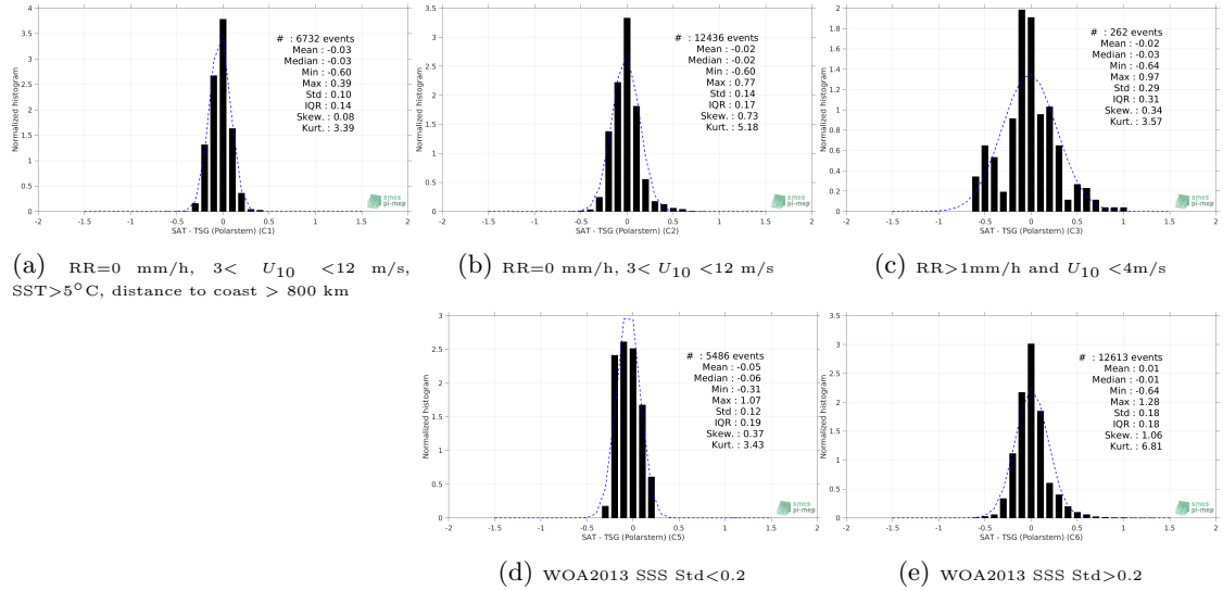
Figure 13: Normalized histogram of \Delta SSS (SMAP SSS L4 OI v1 - 7day (IPRC) - TSG (Polarstern)) for 5 different subdatasets corresponding to: RR=0 mm/h, 3 < U_{10} < 12 m/s, SST > 5^\circ C , distance to coast > 800 km (a), RR=0 mm/h, 3 < U_{10} < 12 m/s (b), RR > 1 mm/h and U_{10} < 4 m/s (c), WOA2013 SSS Std < 0.2 (d), WOA2013 SSS Std > 0.2 (e).
