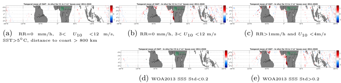
Figure 12: Temporal mean gridded over spatial boxes of size 1^\circ \times 1^\circ of \Delta SSS (SMAP SSS L4 OI v1 - 7 Days (IPRC) - TSG (LEGOS-DM)) for 5 different subdatasets corresponding to:RR=0 mm/h, 3 < U_{10} < 12 m/s, SST>5°C, distance to coast > 800 km (a), RR=0 mm/h, 3 < U_{10} < 12 m/s (b), RR>1mm/h and U_{10} < 4 m/s (c), WOA2013 SSS Std<0.2 (d), WOA2013 SSS Std>0.2 (e).
