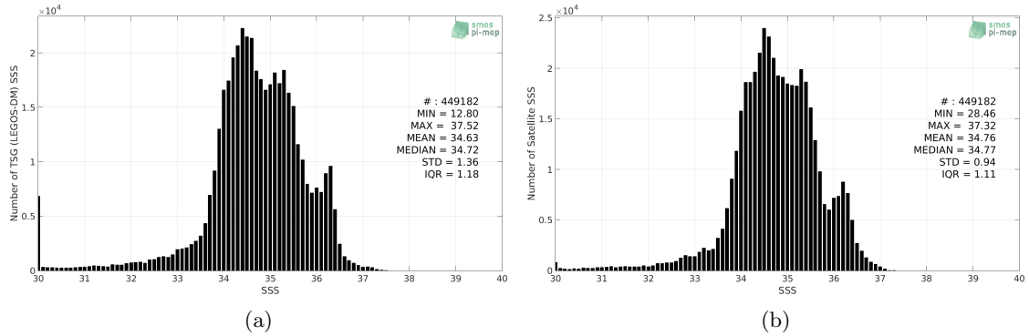
Figure 2: Histograms of SSS from TSG (LEGOS-DM) (a) and SMAP SSS L4 OI v1 - 7 Days (IPRC) (b) considering all match-up pairs per bins of 0.1 over the Equatorial Ocean 10N-10S Pi-MEP region and for the full satellite product period.
