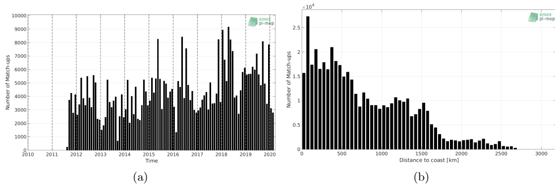
Figure 1: Number of match-ups between TSG (LEGOS-DM) and SMAP SSS L4 OI v1 - 7 Days (IPRC) SSS as a function of time (a) and as function of the distance to coast (b) over the Equatorial Ocean 10N-10S Pi-MEP region and for the full satellite product period.
