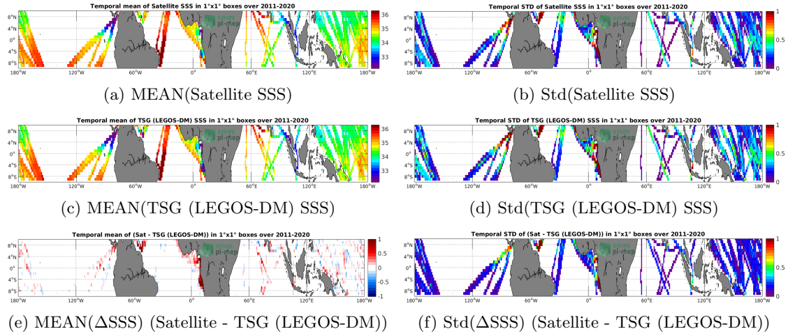
Figure 6: Temporal mean (left) and Std (right) of SSS from SMAP SSS L4 OI v1 - 7 Days (IPRC) (top), TSG (LEGOS-DM) (middle), and of \Delta SSS (Satellite - TSG (LEGOS-DM)). Only match-up pairs are used to generate these maps.
