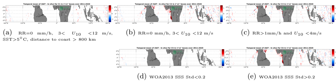
Figure 12: Temporal mean gridded over spatial boxes of size 1°x1° of \Delta SSS (SMAP SSS L4 OI v1 - 7day (IPRC) - TSG (LEGOS-DM)) for 5 different subdatasets corresponding to:RR=0 mm/h, 3 < U_{10} < 12 m/s, SST>5°C, distance to coast > 800 km (a), RR=0 mm/h, 3 < U_{10} < 12 m/s (b), RR>1mm/h and U_{10} < 4 m/s (c), WOA2013 SSS Std<0.2 (d), WOA2013 SSS Std>0.2 (e).
