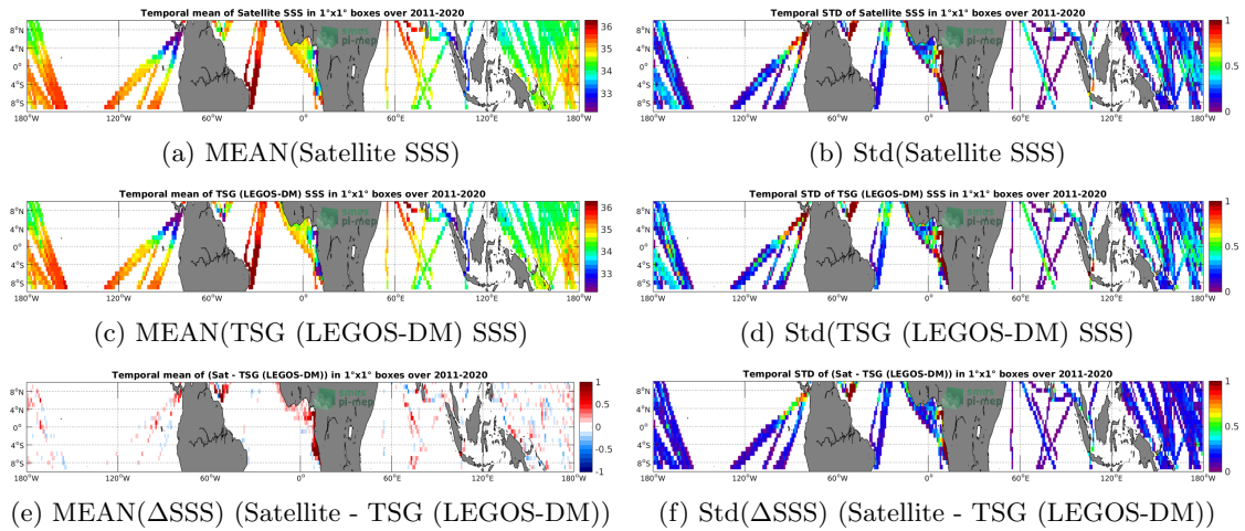
Figure 6: Temporal mean (left) and Std (right) of SSS from SMAP SSS L4 OI v1 - 7day (IPRC) (top), TSG (LEGOS-DM) (middle), and of \Delta SSS (Satellite - TSG (LEGOS-DM)). Only match-up pairs are used to generate these maps.
