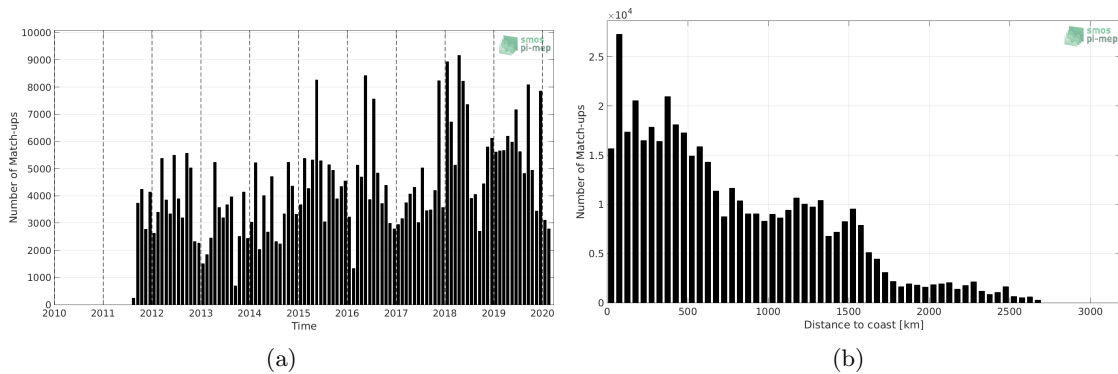
Figure 1: Number of match-ups between TSG (LEGOS-DM) and SMAP SSS L4 OI v1 - 7day (IPRC) SSS as a function of time (a) and as function of the distance to coast (b) over the Equatorial Ocean 10N-10S Pi-MEP region and for the full satellite product period.
