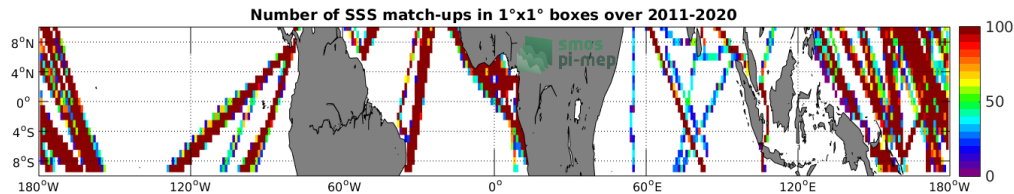
Figure 4: Number of SSS match-ups between TSG (LEGOS-DM) SSS and the SMAP SSS L4 OI v1 - 7day (IPRC) SSS product for the Equatorial Ocean 10N-10S Pi-MEP region over 1^\circ \times 1^\circ boxes and for the full satellite product period.
