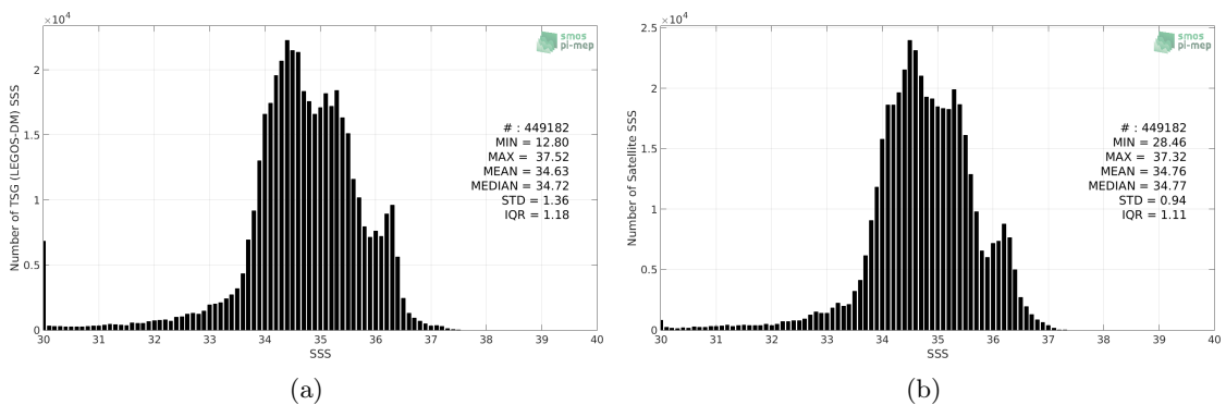
Figure 2: Histograms of SSS from TSG (LEGOS-DM) (a) and SMAP SSS L4 OI v1 - 7day (IPRC) (b) considering all match-up pairs per bins of 0.1 over the Equatorial Ocean 10N-10S Pi-MEP region and for the full satellite product period.
