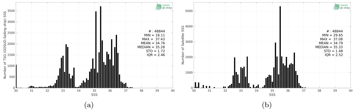
Figure 2: Histograms of SSS from TSG (GOSUD-Sailing-ship) (a) and SMAP SSS L4 OI v1 - 7 Days (IPRC) (b) considering all match-up pairs per bins of 0.1 over the Equatorial Ocean 10N-10S Pi-MEP region and for the full satellite product period.
