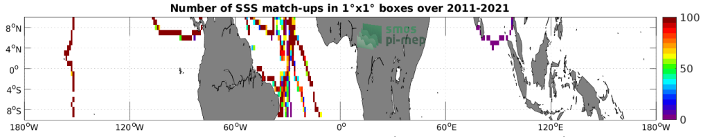
Figure 4: Number of SSS match-ups between TSG (GOSUD-Sailing-ship) SSS and the SMAP SSS L4 OI v1 - 7 Days (IPRC) SSS product for the Equatorial Ocean 10N-10S Pi-MEP region over 1^\circ \times 1^\circ boxes and for the full satellite product period.
