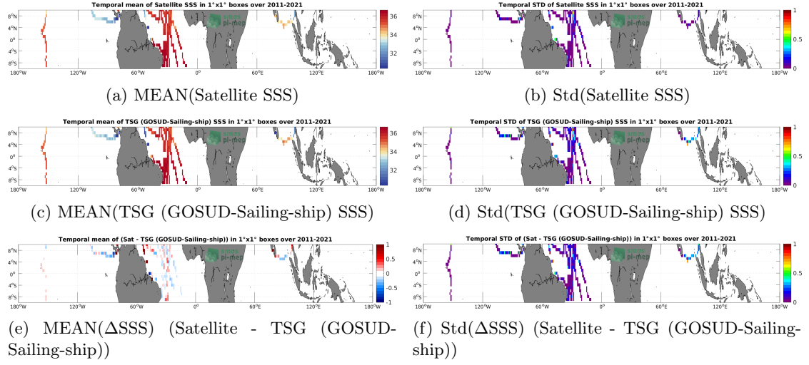
Figure 6: Temporal mean (left) and Std (right) of SSS from SMAP SSS L4 OI v1 - 7 Days (IPRC) (top), TSG (GOSUD-Sailing-ship) (middle), and of \Delta SSS (Satellite - TSG (GOSUD-Sailing-ship)). Only match-up pairs are used to generate these maps.
