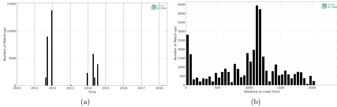
Figure 1: Number of match-ups between TSG (GOSUD-Sailing-ship) and SMAP SSS L4 OI v1 - 7day (IPRC) SSS as a function of time (a) and as function of the distance to coast (b) over the Equatorial Ocean 10N-10S Pi-MEP region and for the full satellite product period.
